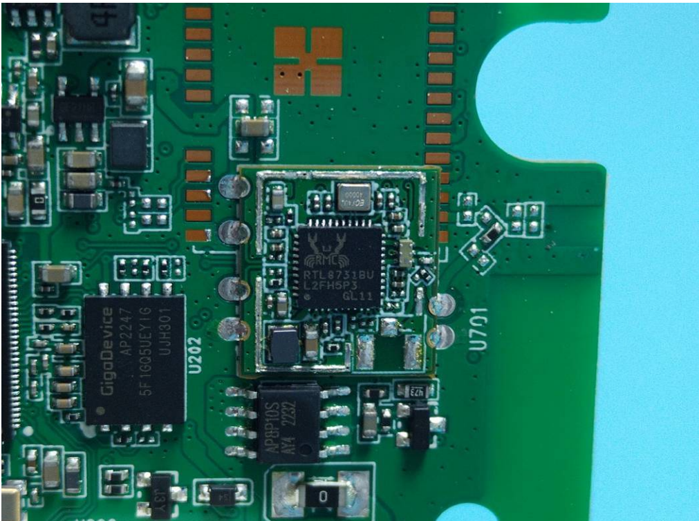
WIFI Chip
