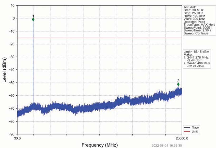
Pi/4DQPSK_2DH5_MCH_2441MHz_Ant1_NTNV
