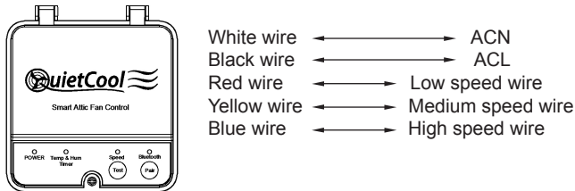
Fig. 2 Connection Wires of IT-AF-SMT
