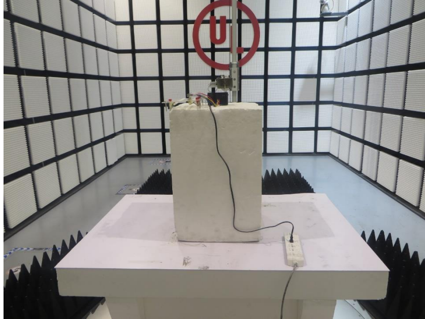
MEASUREMENT POSITION
