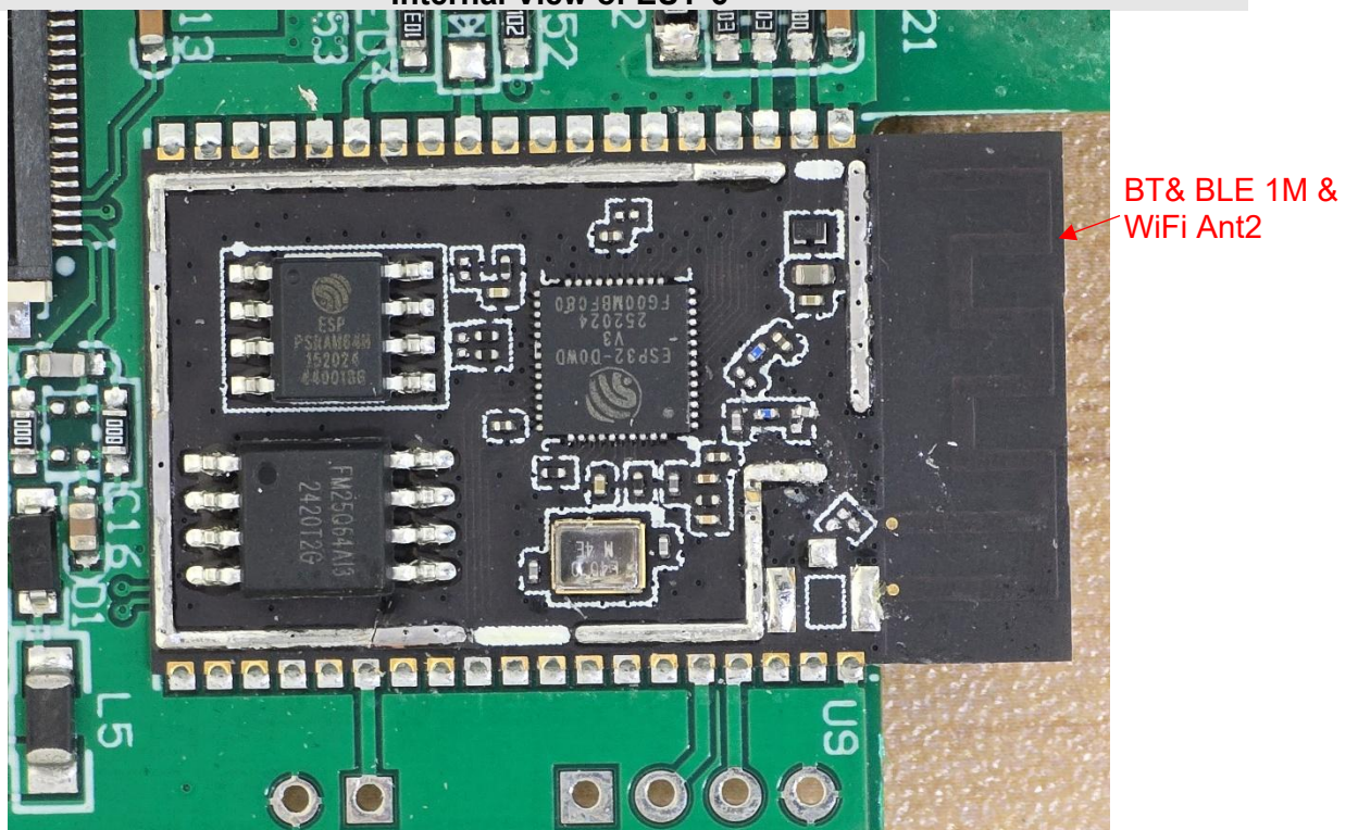
Internal View of EUT-6
