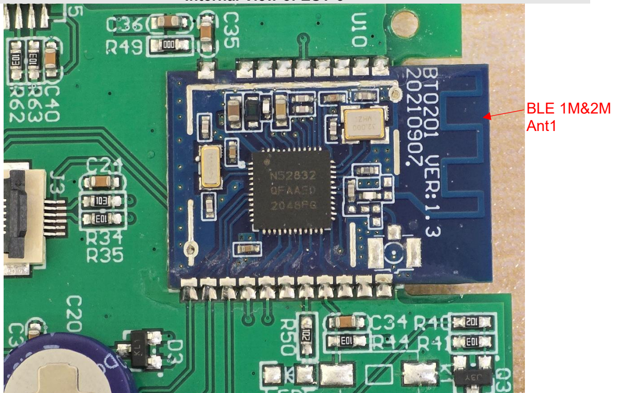
Internal View of EUT-6
