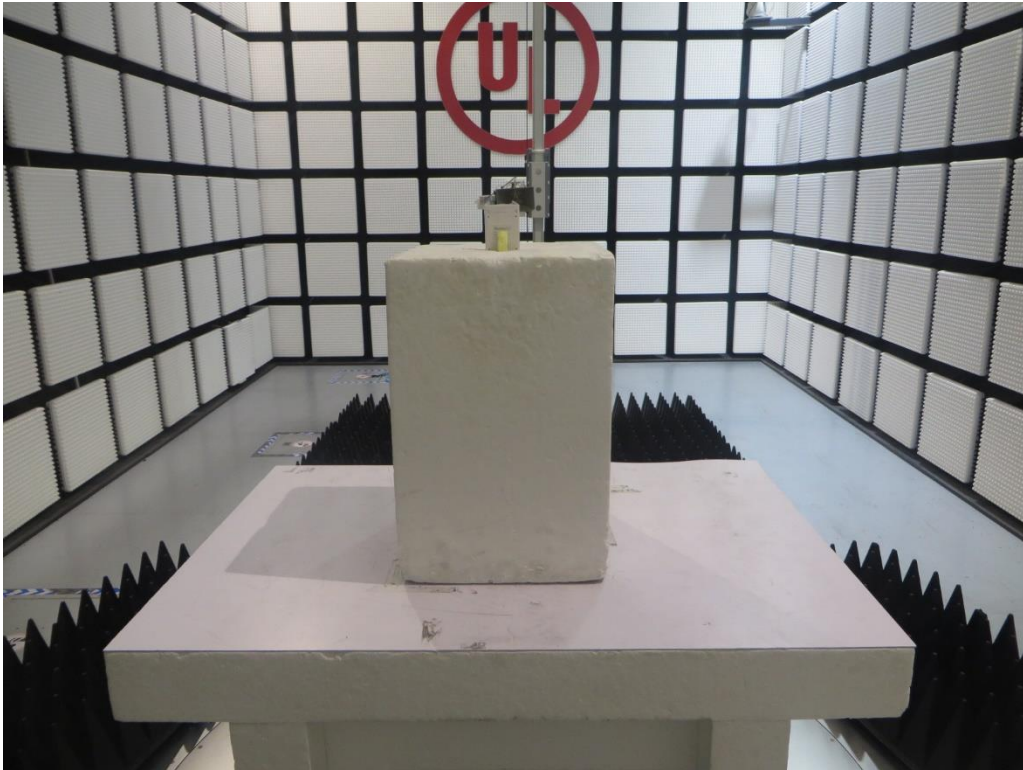
Radiated Disturbance Setup
