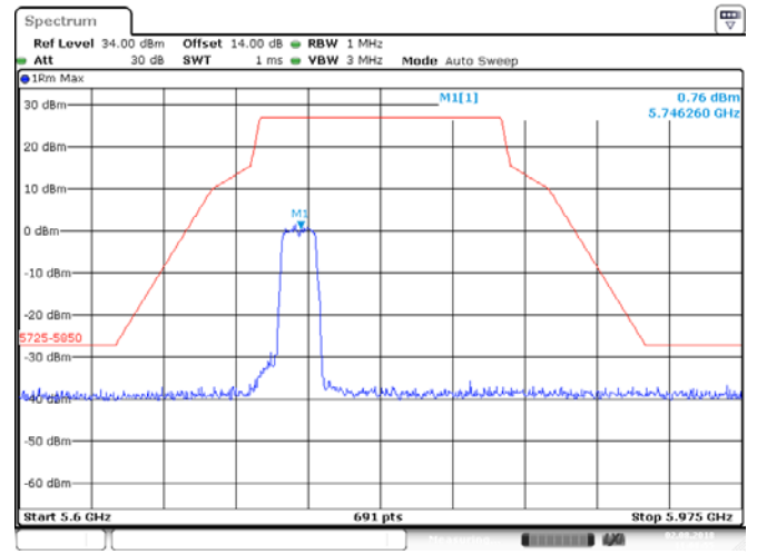
ANT 2(11N) 5745MHz
