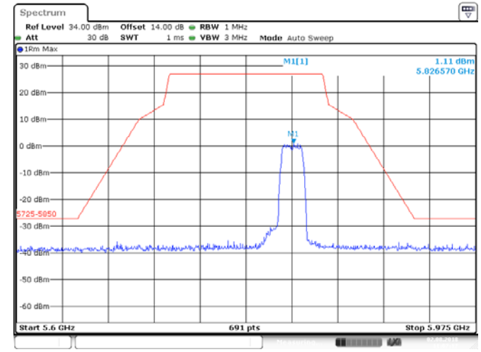
ANT 2(11N) 5825MHz
