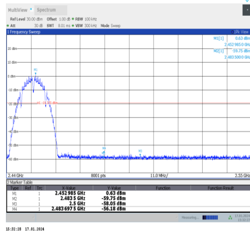
11b-Ant1-2452-PASS
