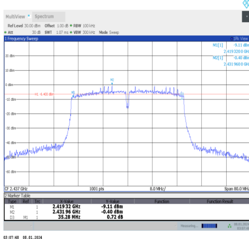
11n40MIMO-Ant0-2437-PASS
