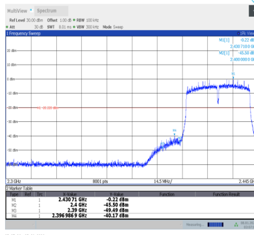
11n40MIMO-Ant1-2422-PASS
