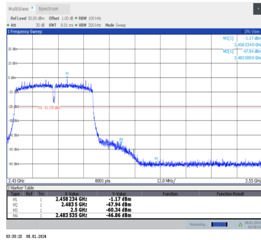
11n40MIMO-Ant1-2452-PASS
