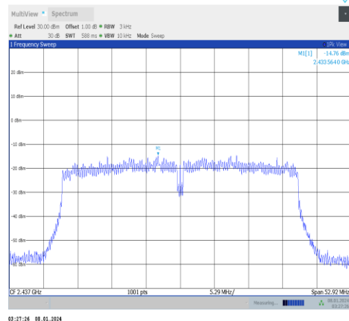
11n40MIMO-Ant1-2437-PASS
