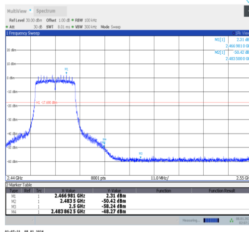
11n20MIMO-Ant1-2462-PASS
