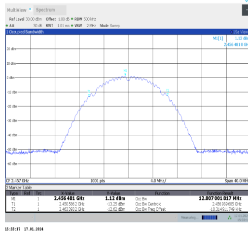
11b-Ant1-2457
