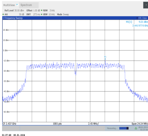
11g-Ant1-2437-PASS
