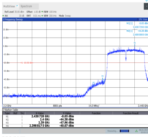
11n40MIMO-Ant0-2422-PASS
