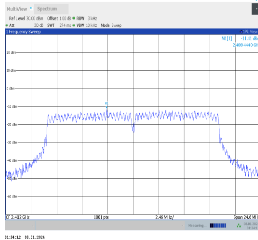
11g-Ant1-2412-PASS
