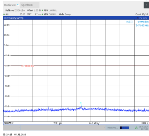
11n40MIMO-Ant0-2452-30~1000-PASS
