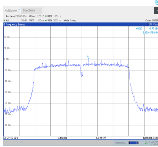
11n40MIMO-Ant1-2427-0~Reference-PASS
