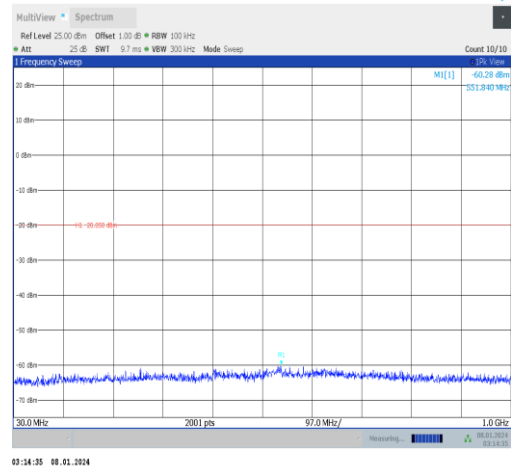
11n40MIMO-Ant0-2437-30~1000-PASS
