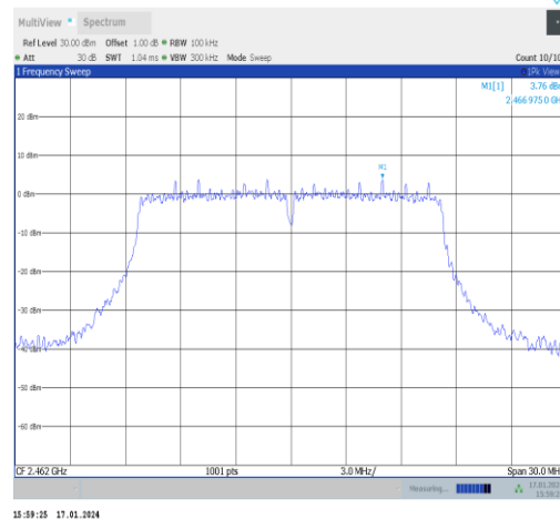
11g-Ant1-2462-0~Reference-PASS
