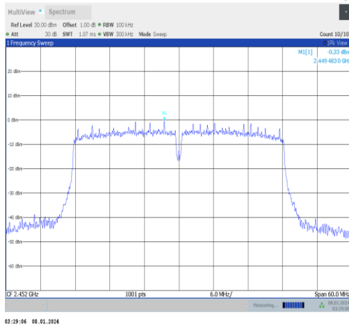
11n40MIMO-Ant0-2452-0~Reference-PASS
