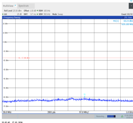
11b-Ant1-2437-30~1000-PASS
