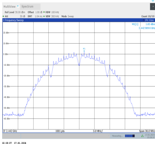
11b-Ant1-2442-0~Reference-PASS
