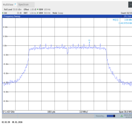
11n20MIMO-Ant0-2437-0~Reference-PASS
