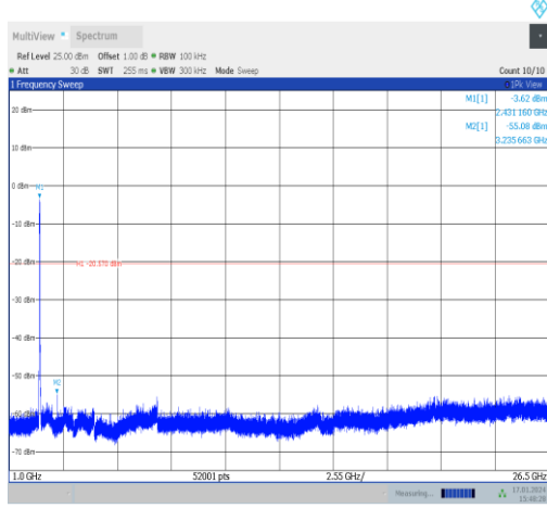
11n40MIMO-Ant0-2427-1000~26500-PASS
