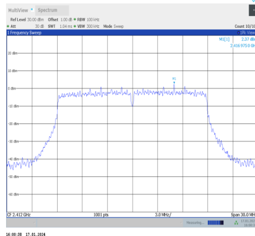
11n20MIMO-Ant1-2412-0~Reference-PASS
