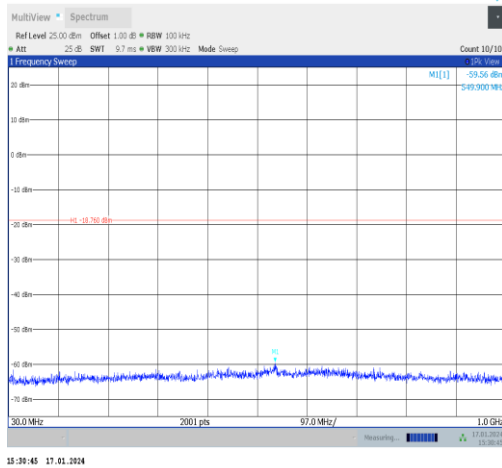
11b-Ant1-2447-30~1000-PASS
