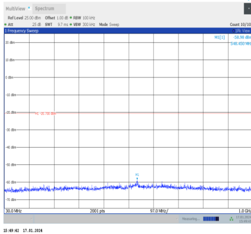
11n40MIMO-Ant1-2427-30~1000-PASS
