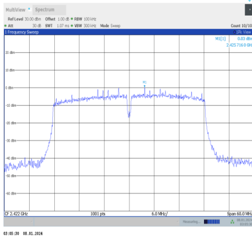
11n40MIMO-Ant0-2422-0~Reference-PASS
