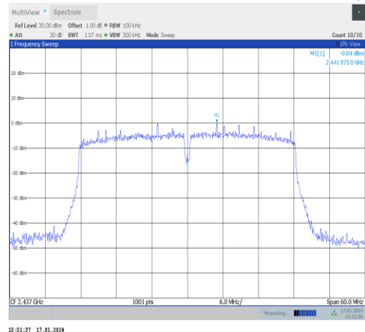
11n40MIMO-Ant1-2437-0~Reference-PASS
