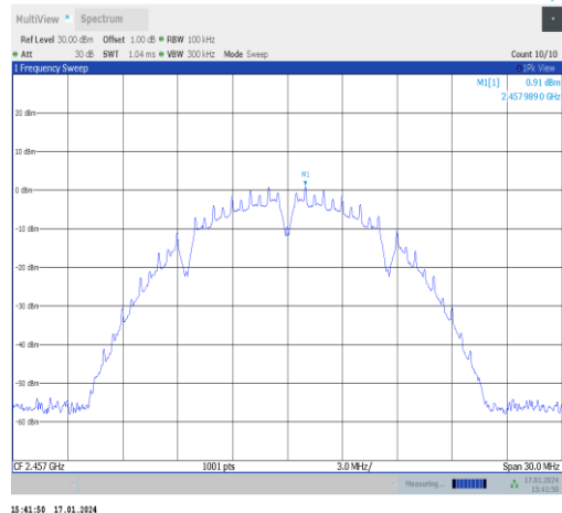
11b-Ant1-2457-0~Reference-PASS
