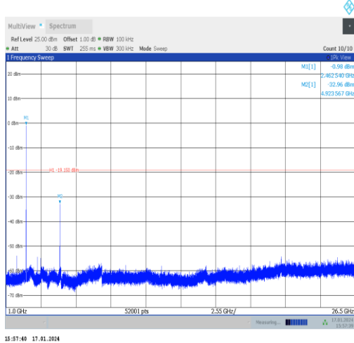
11b-Ant1-2462-1000~26500-PASS
