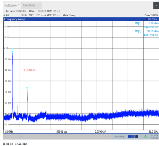
11n40MIMO-Ant1-2437-1000~26500-PASS
