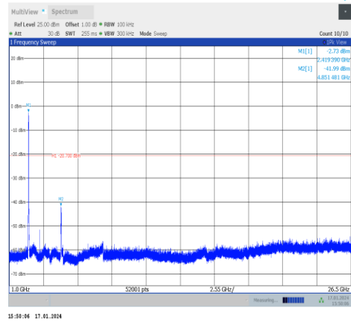
11n40MIMO-Ant1-2427-1000~26500-PASS
