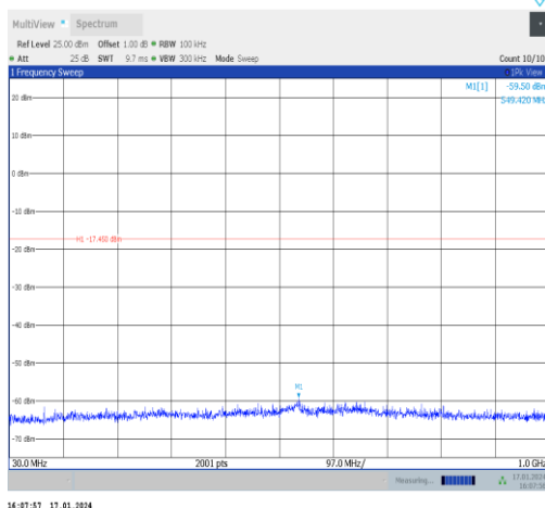
11n20MIMO-Ant1-2437-30~1000-PASS
