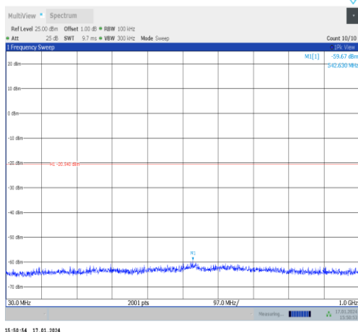
11n40MIMO-Ant1-2422-30~1000-PASS
