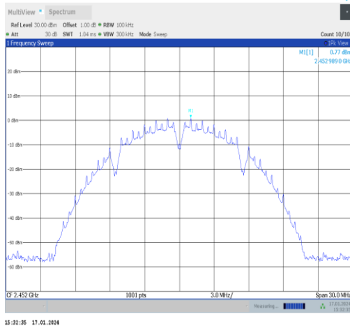
11b-Ant1-2452-0~Reference-PASS
