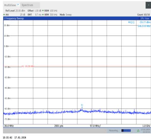
11b-Ant1-2452-30~1000-PASS
