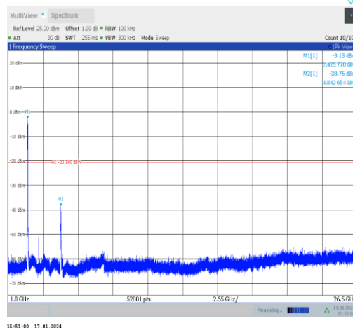
11n40MIMO-Ant1-2422-1000~26500-PASS
