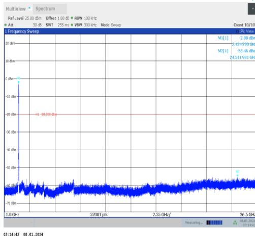
11n40MIMO-Ant0-2437-1000~26500-PASS
