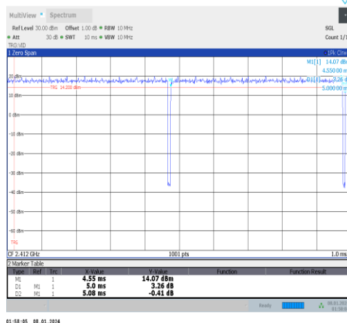
NTNV-11n20MIMO-Ant1-2412
