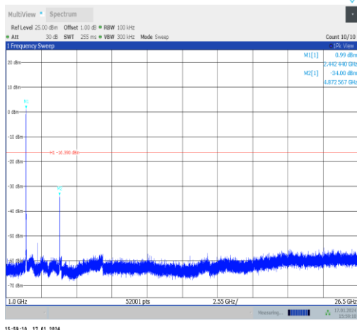
11g-Ant1-2437-1000~26500-PASS
