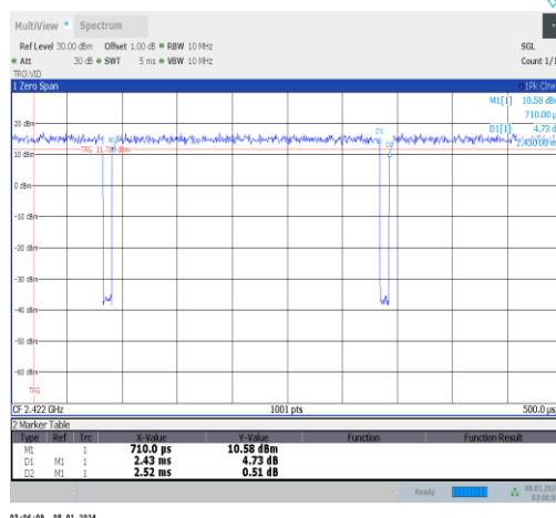
NTNV-11n40MIMO-Ant1-2422
