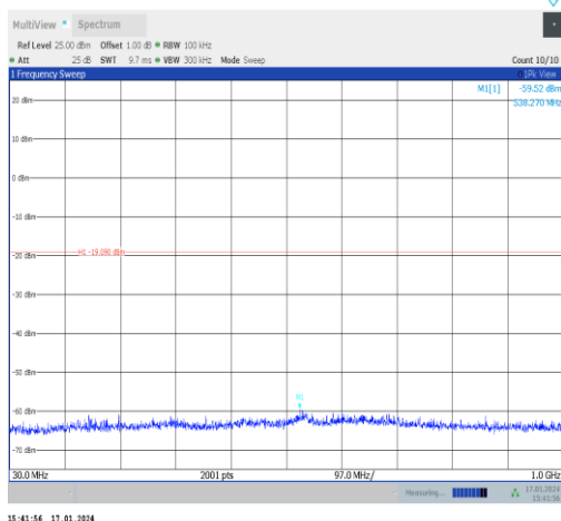
11b-Ant1-2457-30~1000-PASS
