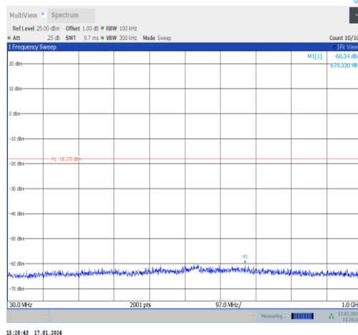
11b-Ant1-2442-30~1000-PASS
