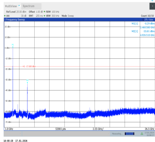
11n20MIMO-Ant1-2462-1000~26500-PASS
