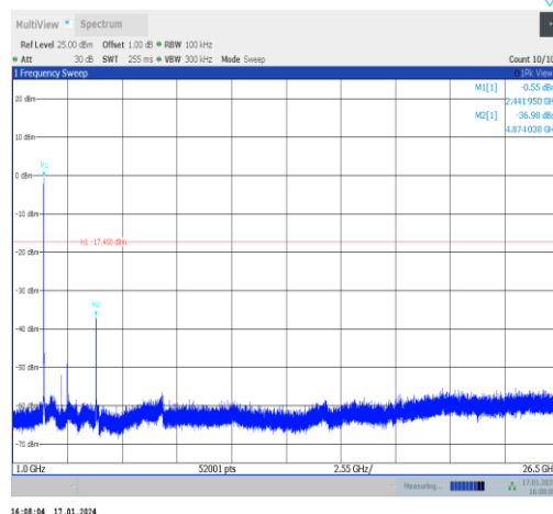
11n20MIMO-Ant1-2437-1000~26500-PASS
