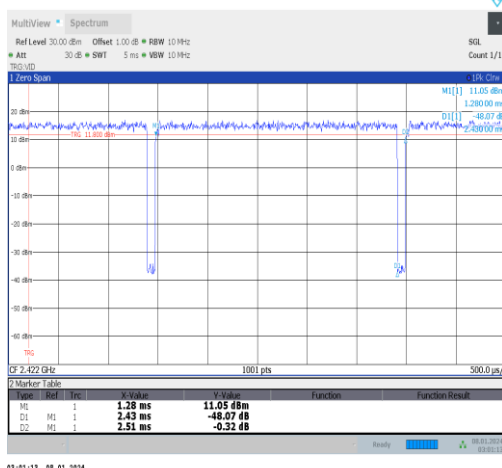
NTNV-11n40MIMO-Ant0-2422
