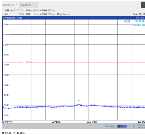
11n20MIMO-Ant1-2412-30~1000-PASS
