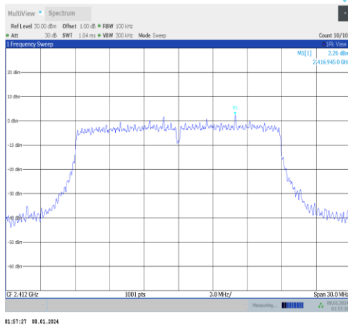
11n20MIMO-Ant0-2412-0~Reference-PASS
