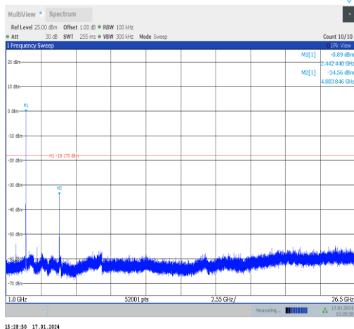
11b-Ant1-2442-1000~26500-PASS
