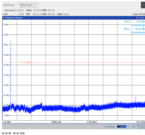
11n20MIMO-Ant0-2437-1000~26500-PASS
