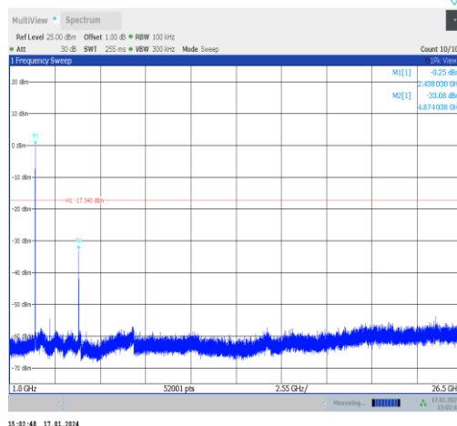
11b-Ant1-2437-1000~26500-PASS
