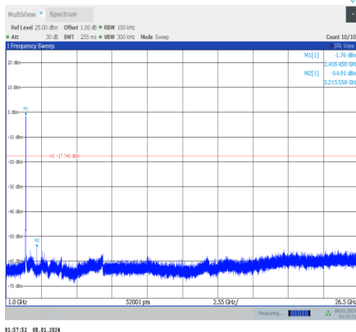
11n20MIMO-Ant0-2412-1000~26500-PASS
