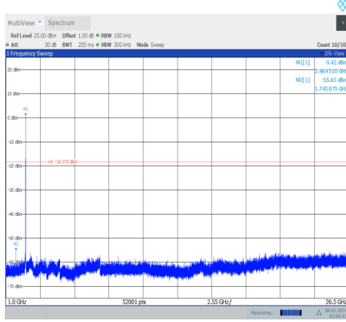
11n20MIMO-Ant0-2462-1000~26500-PASS
