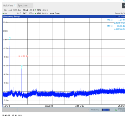
11b-Ant1-2457-1000~26500-PASS
