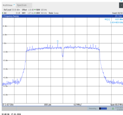
11n40MIMO-Ant0-2427-0~Reference-PASS
