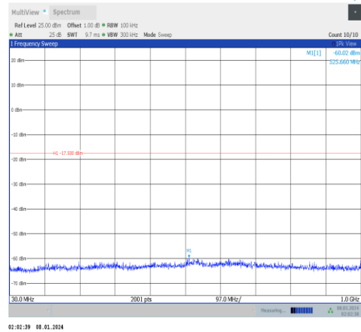
11n20MIMO-Ant0-2437-30~1000-PASS
