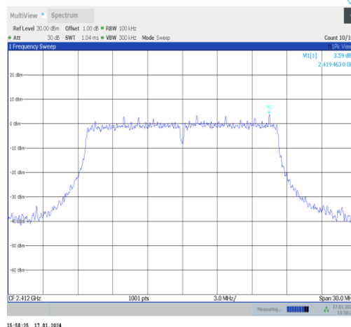
11g-Ant1-2412-0~Reference-PASS
