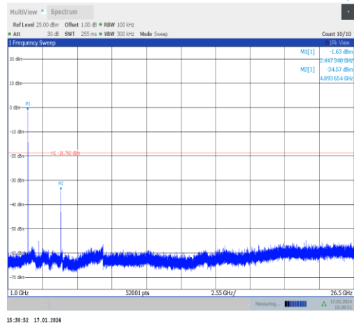
11b-Ant1-2447-1000~26500-PASS
