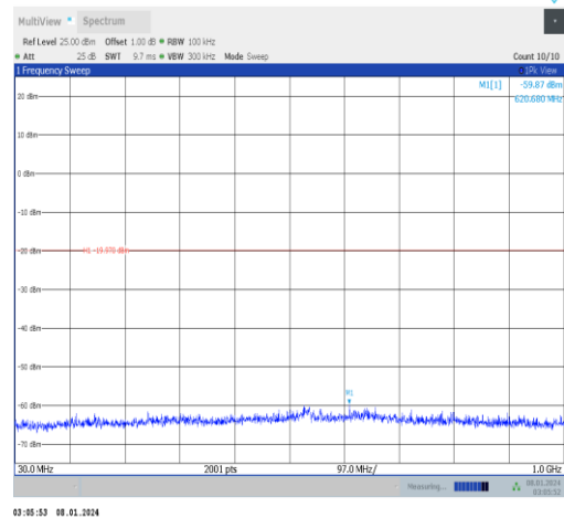
11n40MIMO-Ant0-2422-30~1000-PASS
