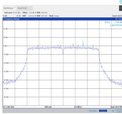
11n20MIMO-Ant1-2462-0~Reference-PASS
