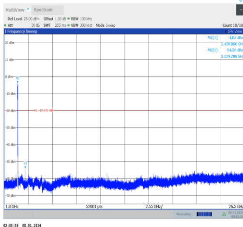
11n40MIMO-Ant0-2422-1000~26500-PASS
