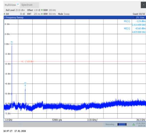
11n20MIMO-Ant1-2412-1000~26500-PASS
