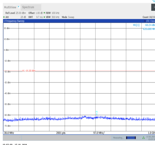
11b-Ant1-2462-30~1000-PASS
