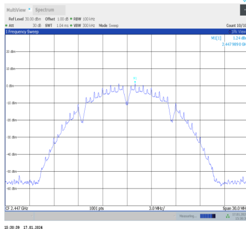
11b-Ant1-2447-0~Reference-PASS
