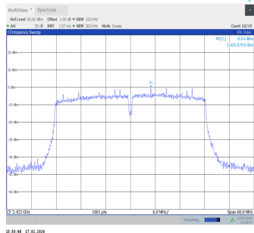
11n40MIMO-Ant1-2422-0~Reference-PASS
