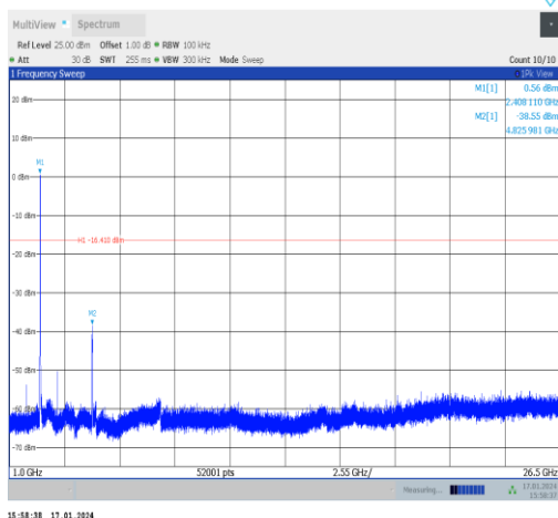
11g-Ant1-2412-1000~26500-PASS
