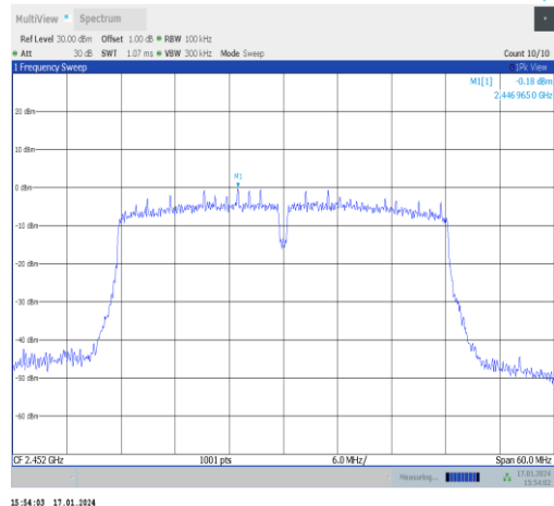
11n40MIMO-Ant1-2452-0~Reference-PASS
