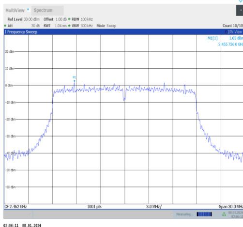
11n20MIMO-Ant0-2462-0~Reference-PASS
