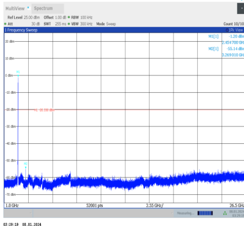
11n40MIMO-Ant0-2452-1000~26500-PASS
