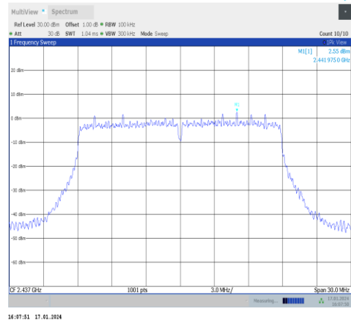
11n20MIMO-Ant1-2437-0~Reference-PASS
