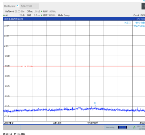
11n40MIMO-Ant0-2427-30~1000-PASS
