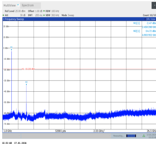
11b-Ant1-2452-1000~26500-PASS
