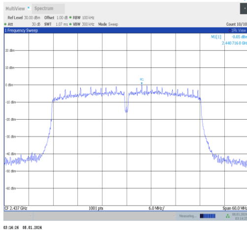
11n40MIMO-Ant0-2437-0~Reference-PASS
