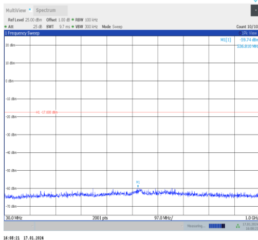
11n20MIMO-Ant1-2462-30~1000-PASS
