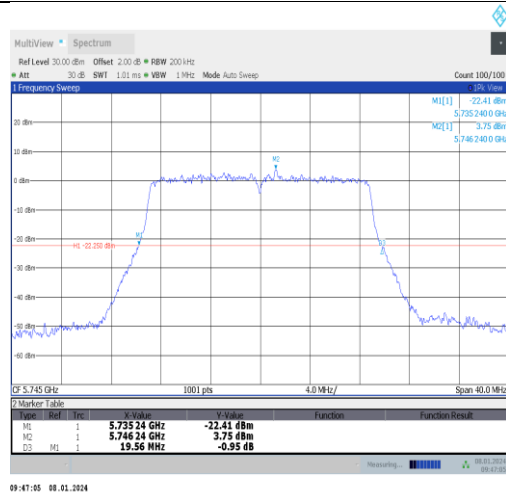
11ac20MIMO-Ant0-5745
