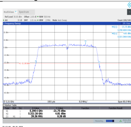
11ac40MIMO-Ant0-5310
