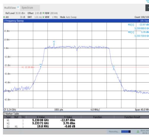
11ac20MIMO-Ant0-5240
