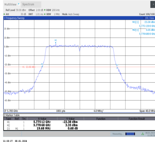
11ac20MIMO-Ant0-5785
