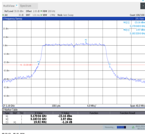
11ac20MIMO-Ant1-5180
