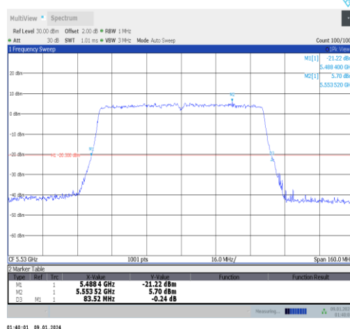
11ac80MIMO-Ant0-5530
