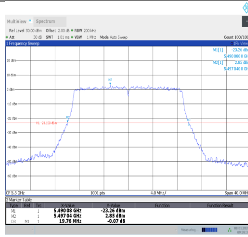
11ac20MIMO-Ant0-5500
