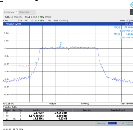
11ac20MIMO-Ant0-5180
