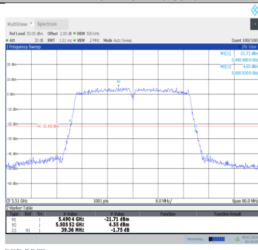
11ac40MIMO-Ant0-5510
