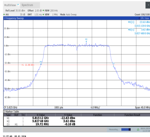
11ac20MIMO-Ant0-5825
