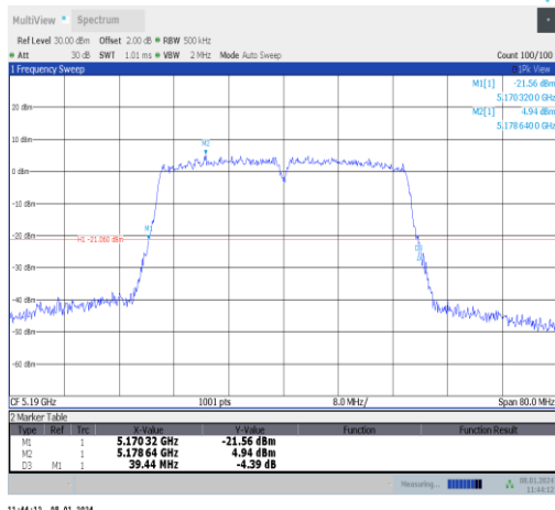
11ac40MIMO-Ant1-5190
