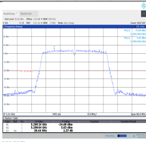
11ac40MIMO-Ant1-5310
