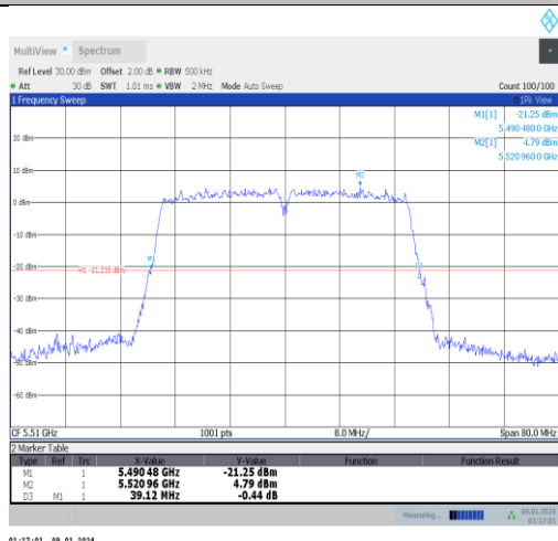
11ac40MIMO-Ant1-5510
