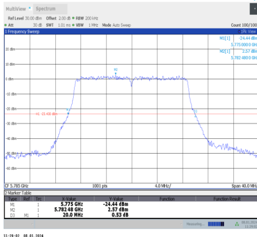
11ac20MIMO-Ant1-5785
