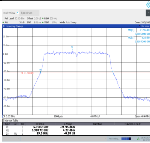
11ac20MIMO-Ant1-5320
