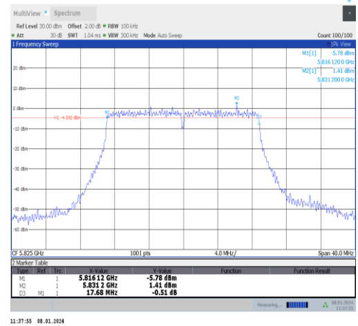
11ac20MIMO-Ant0-5825-PASS
