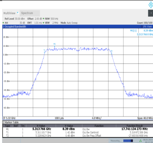
11ac20MIMO-Ant1-5320
