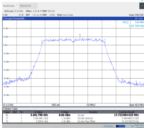
11ac20MIMO-Ant1-5500
