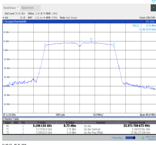
11ac40MIMO-Ant1-5190
