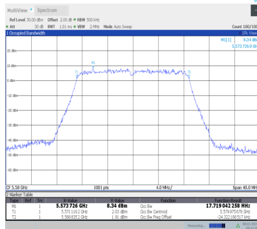
11ac20MIMO-Ant0-5580
