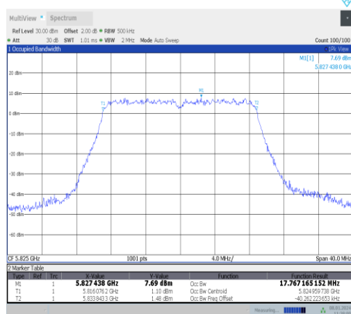
11ac20MIMO-Ant0-5825
