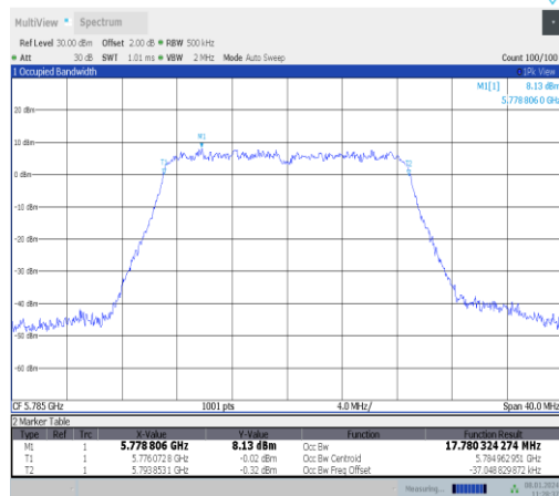
11ac20MIMO-Ant0-5785
