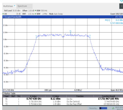
11ac20MIMO-Ant0-5745
