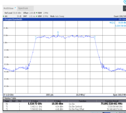
11ac80MIMO-Ant0-5530
