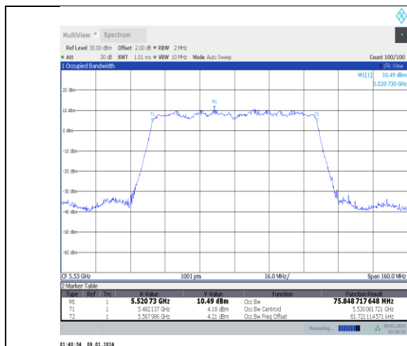
11ac80MIMO-Ant1-5530
