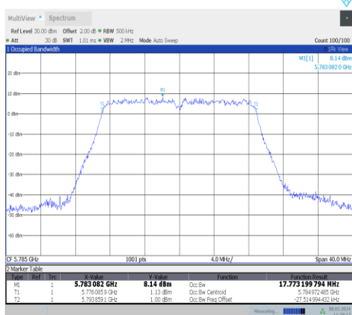
11ac20MIMO-Ant1-5785
