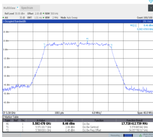
11ac20MIMO-Ant1-5580
