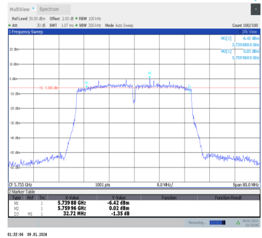
11ac40MIMO-Ant0-5755-PASS
