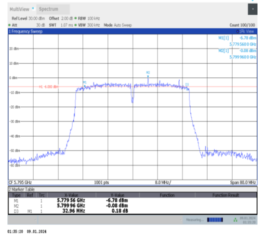
11ac40MIMO-Ant0-5795-PASS
