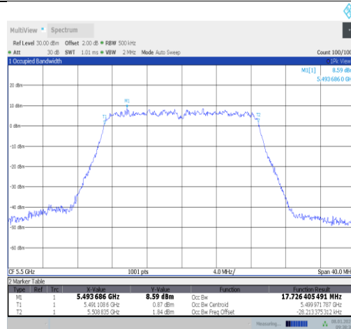
11ac20MIMO-Ant0-5500
