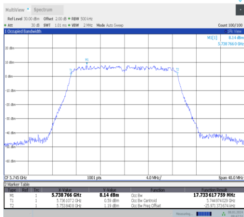
11ac20MIMO-Ant1-5745
