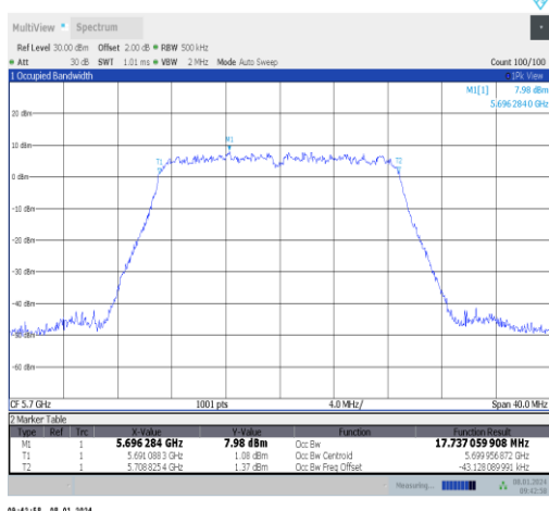
11ac20MIMO-Ant1-5700
