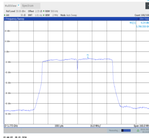
11ac80MIMO-Ant1-5775-PASS
