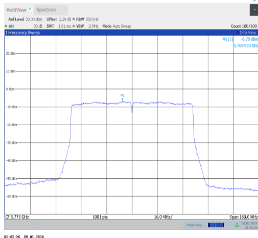
11ac80MIMO-Ant0-5775-PASS
