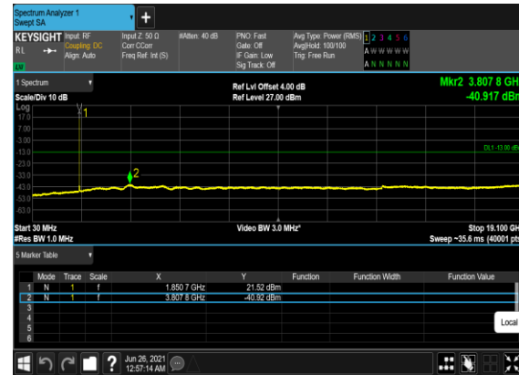
B5_N2(5M)_DFT-s- OFDM_QPSK_Edge_1RB_Left_Low_CH
