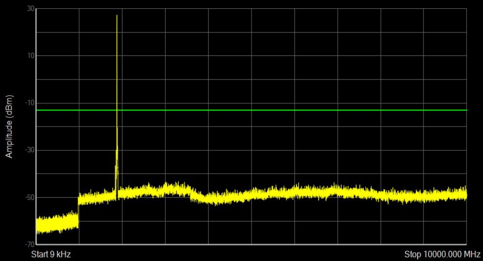
Band25 QAM16 BW=20MHz Channel=26590 RB Size=1 Position=#0
