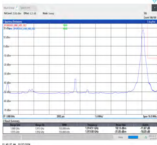
1-N25-15-15-H-5-CP-QPSK-Edge_1RB_Right-1@78-Ant4-1-seegraph-PASS-see graph
