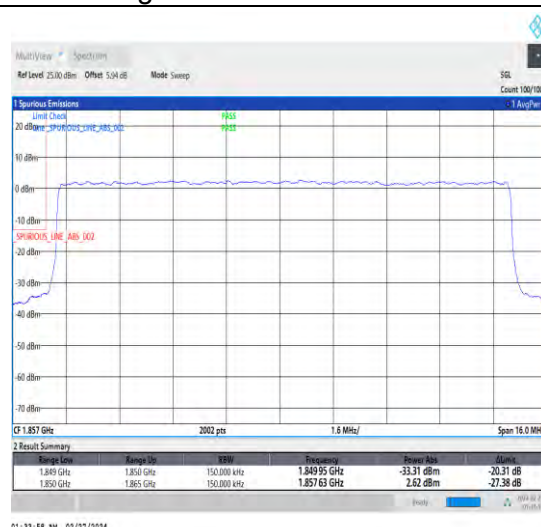
1-N25-15-15-L-3-DFT-PI2BPSK-Outer_Full-75@0-Ant4-1-seegraph-PASS-see graph
