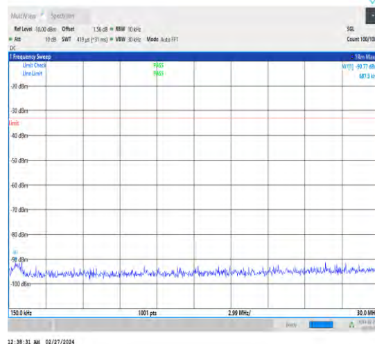
1-N25-15-20-L-1-DFT-PI2BPSK-Inner_1RB_Left-1@ 1-0.15-30-Ant4-0.69--90.77--33-PASS
