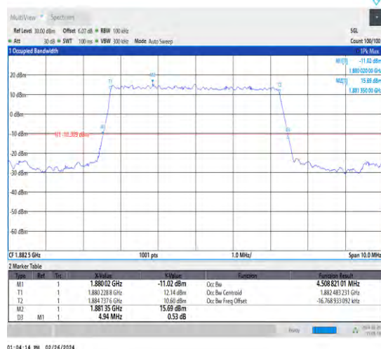
1-N25-15-5-M-2-DFT-PI2BPSK-Outer_Full-25@0-An t4-4.509-4.940-≤5-PASS
