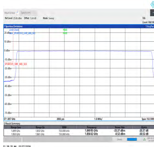
1-N25-15-15-L-6-CP-QPSK-Outer_Full-79@0-Ant4-1-seegraph-PASS-see graph
