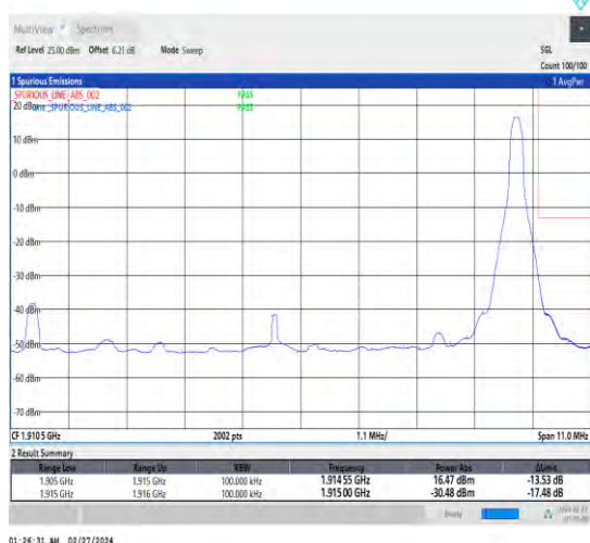
1-N25-15-10-H-5-CP-QPSK-Edge_1RB_Right-1@51-Ant4-1-seegraph-PASS-see graph
