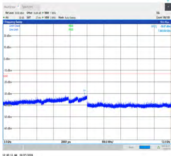
1-N25-15-20-H-1-DFT-PI2BPSK-Inner_1RB_Left-1 @1-3000-12000-Ant4-7360.05--30.87--13-PASS
