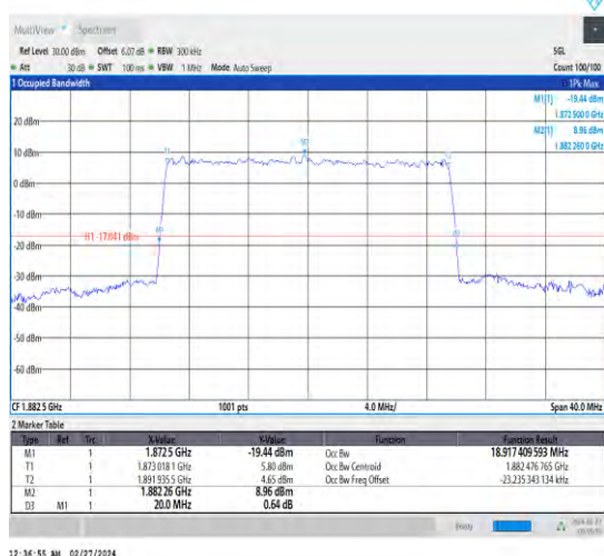
1-N25-15-20-M-9-CP-256QAM-Outer_Full-106@0-Ant4 -18.917-20.000-≤20-PASS
