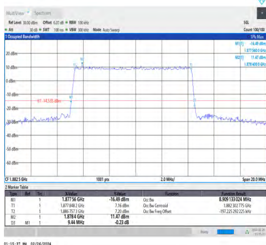
1-N25-15-10-M-3-DFT-16QAM-Outer_Full-50@0-Ant 4-8.909-9.440-≤10-PASS
