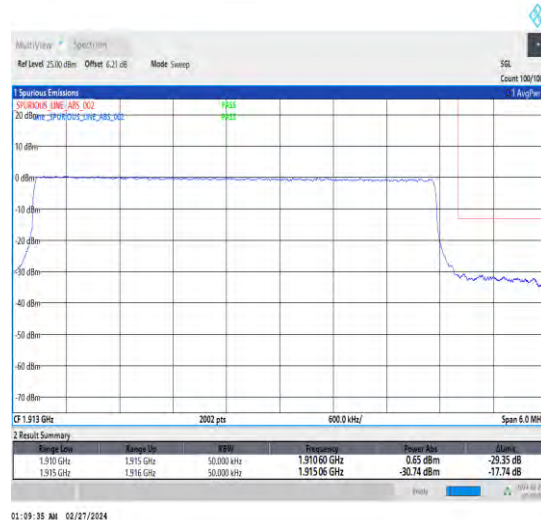
1-N25-15-5-H-6-CP-QPSK-Outer_Full-25@0-Ant4-1 1-seegraph-PASS-see graph
