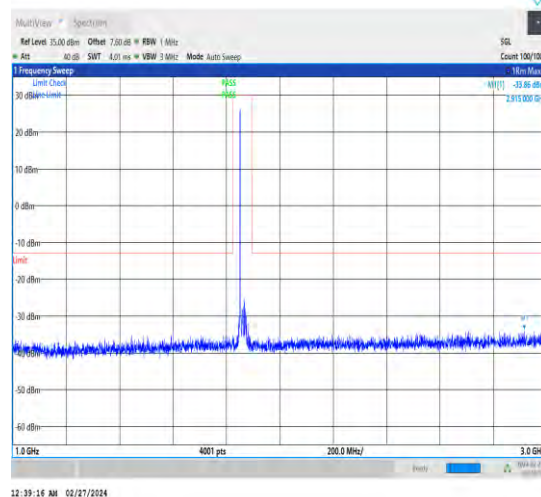
1-N25-15-20-L-1-DFT-PI2BPSK-Inner_1RB_Left-1@ 1-1000-3000-Ant4-2915.00--33.86--13-PASS
