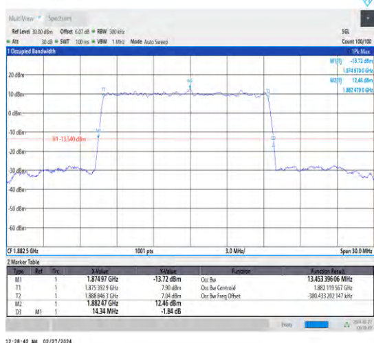
1-N25-15-15-M-5-DFT-256QAM-Outer_Full-75@0-A nt4-13.453-14.340≤15-PASS
