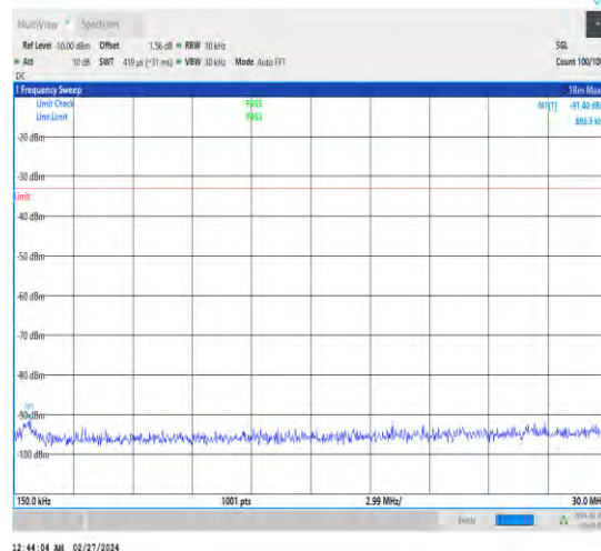
1-N25-15-20-H-1-DFT-PI2BPSK-Inner_1RB_Left-1@ 1-0.15-30-Ant4-0.90--91.40--33-PASS
