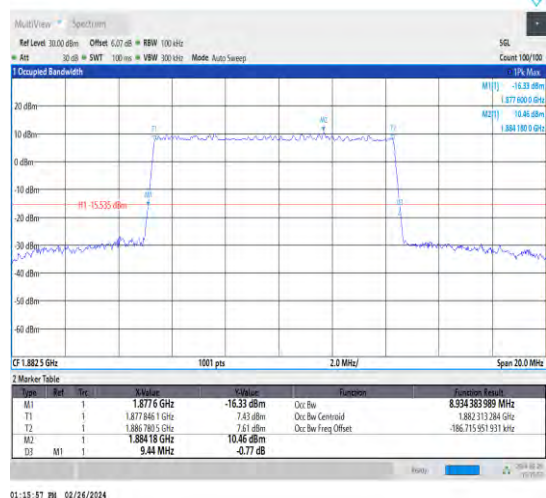
1-N25-15-10-M-4-DFT-64QAM-Outer_Full-50@0-Ant 4-8.934-9.440-≤10-PASS
