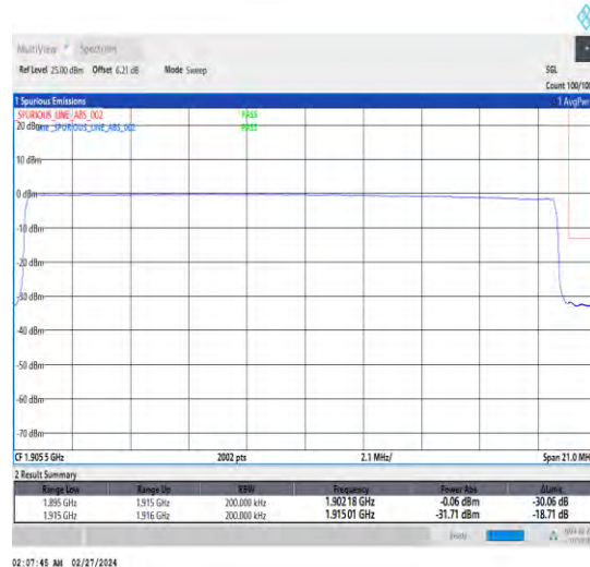
1-N25-15-20-H-6-CP-QPSK-Outer_Full-106@0-Ant4-1-seegraph-PASS-see graph
