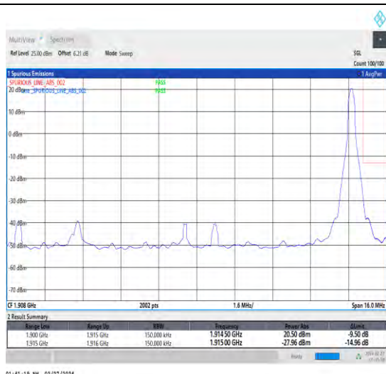
1-N25-15-15-H-2-DFT-PI2BPSK-Edge_1RB_Right-1@78-Ant4-1-seegraph-PASS-see graph
