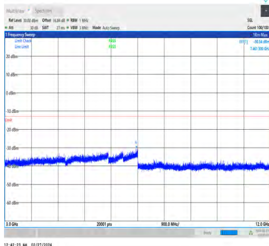
1-N25-15-20-M-1-DFT-PI2BPSK-Inner_1RB_Left-1 @1-3000-12000-Ant4-7461.30--30.54--13-PASS
