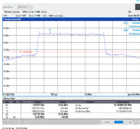
1-N25-15-15-M-6-CP-QPSK-Outer_Full-79@0-Ant4- 14.15-15.030≤15-PASS
