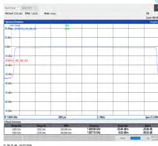
1-N25-15-20-L-6-CP-QPSK-Outer_Full-106@0-Ant4-1-seegraph-PASS-see graph
