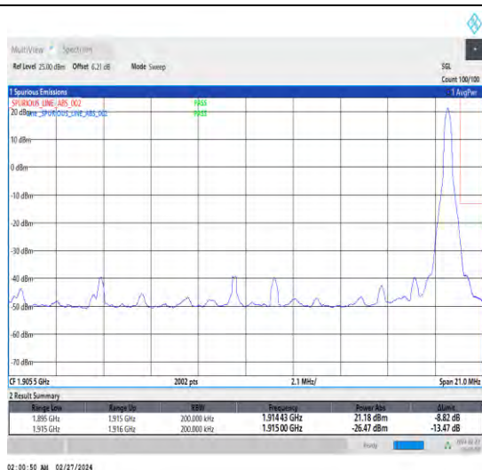
1-N25-15-20-H-2-DFT-PI2BPSK-Edge_1RB_Right-1@105-Ant4-1-seegraph-PASS-see graph
