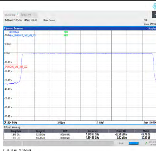
1-N25-15-10-L-6-CP-QPSK-Outer_Full-52@0-Ant4-1-seegraph-PASS-see graph
