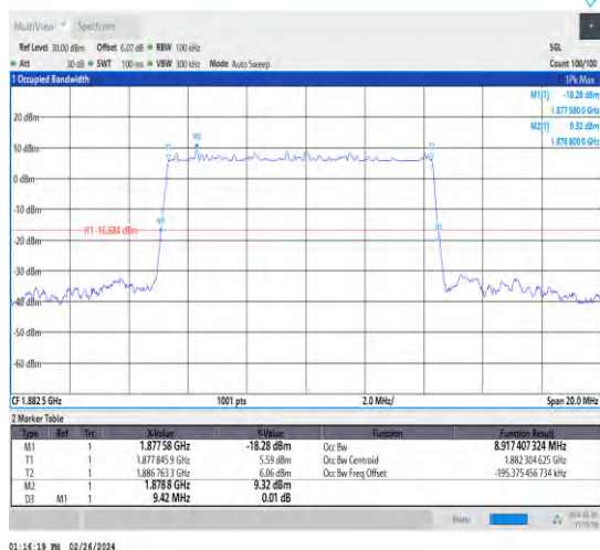
1-N25-15-10-M-5-DFT-256QAM-Outer_Full-50@0-Ant nt4-8.917-9.420-≤10-PASS
