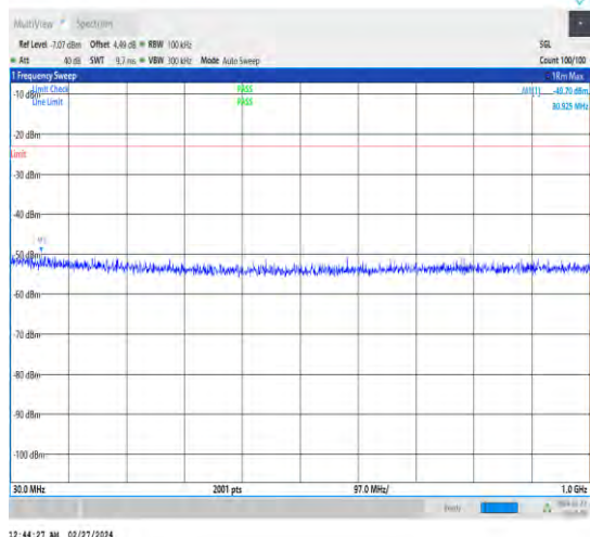
1-N25-15-20-H-1-DFT-PI2BPSK-Inner_1RB_Left-1 @1-30-1000-Ant4-80.93--49.70--23-PASS
