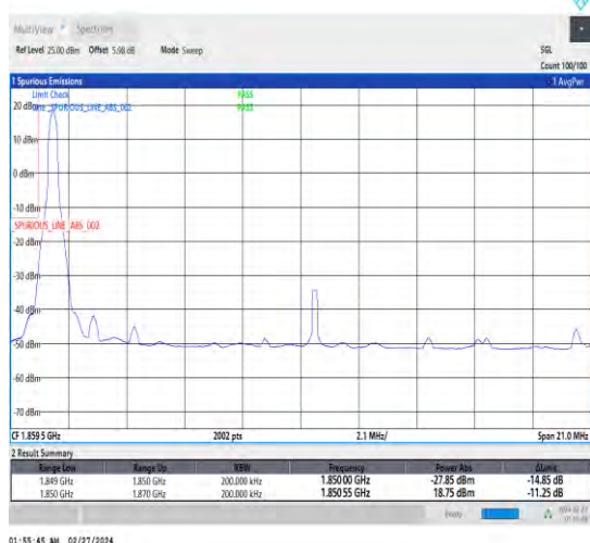
1-N25-15-20-L-4-CP-QPSK-Edge_1RB_Left-1@0-Ant4-1-seegraph-PASS-see graph
