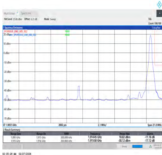
1-N25-15-20-H-5-CP-QPSK-Edge_1RB_Right-1@105-Ant4-1-seegraph-PASS-see graph
