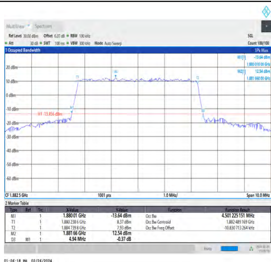
1-N25-15-5-M-7-CP-16QAM-Outer_Full-25@0-Ant4-4 4.501-4.940-≤5-PASS
