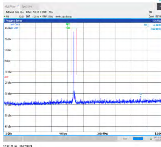
1-N25-15-20-M-1-DFT-PI2BPSK-Inner_1RB_Left-1@ 1-1000-3000-Ant4-2722.00--33.82--13-PASS
