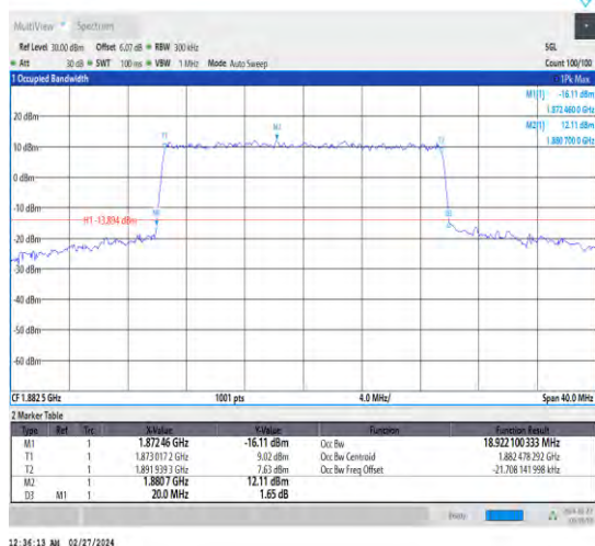
1-N25-15-20-M-7-CP-16QAM-Outer_Full-106@0-Ant4 -18.922-20.000-≤20-PASS
