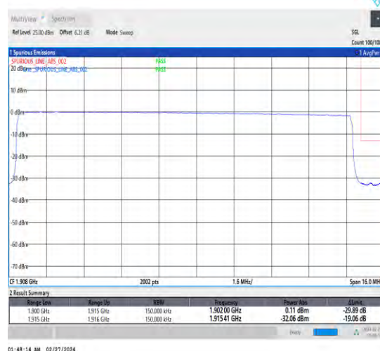
1-N25-15-15-H-6-CP-QPSK-Outer_Full-79@0-Ant4-1-seegraph-PASS-see graph
