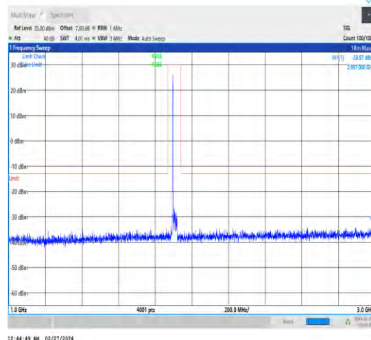
1-N25-15-20-H-1-DFT-PI2BPSK-Inner_1RB_Left-1@ 1-1000-3000-Ant4-2997.00--33.97--13-PASS
