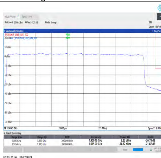
1-N25-15-20-H-3-DFT-PI2BPSK-Outer_Full-100@0-Ant4-1-seegraph-PASS-see graph
