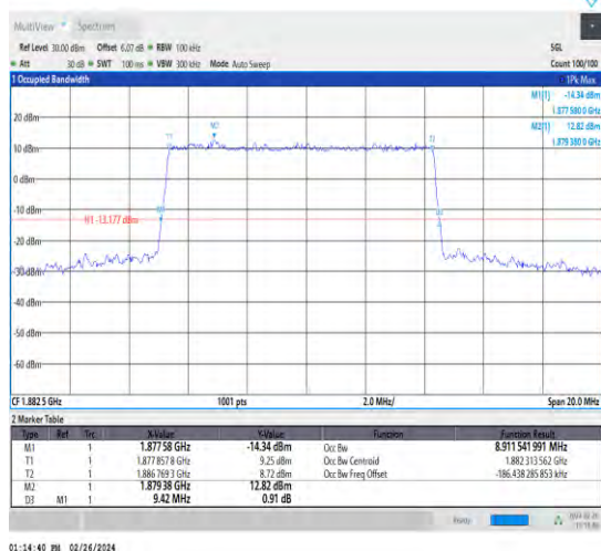
1-N25-15-10-M-1-DFT-QPSK-Outer_Full-50@0-Ant4 -8.912-9.420-≤10-PASS
