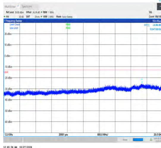
1-N25-15-20-H-1-DFT-PI2BPSK-Inner_1RB_Left-1@ 1-12000-20000-Ant4-18947.60--24.96--13-PASS
