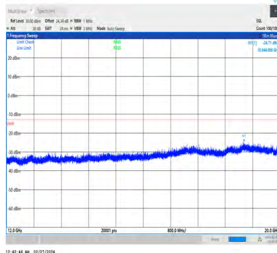
1-N25-15-20-M-1-DFT-PI2BPSK-Inner_1RB_Left-1@ 1-12000-20000-Ant4-18944.00--24.71--13-PASS
