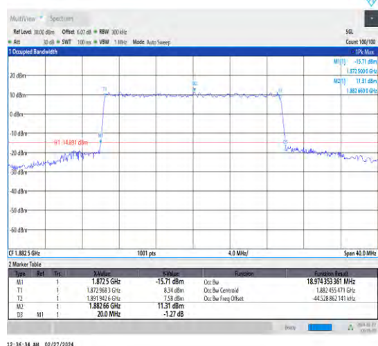
1-N25-15-20-M-8-CP-64QAM-Outer_Full-106@0-Ant4 4-18.974-20.000-≤20-PASS
