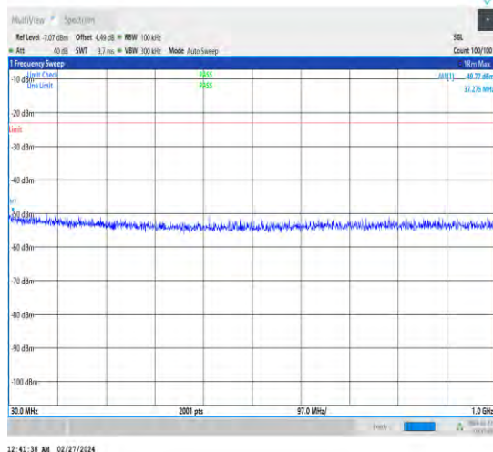
1-N25-15-20-M-1-DFT-PI2BPSK-Inner_1RB_Left-1 @1-30-1000-Ant4-37.28--49.77--23-PASS
