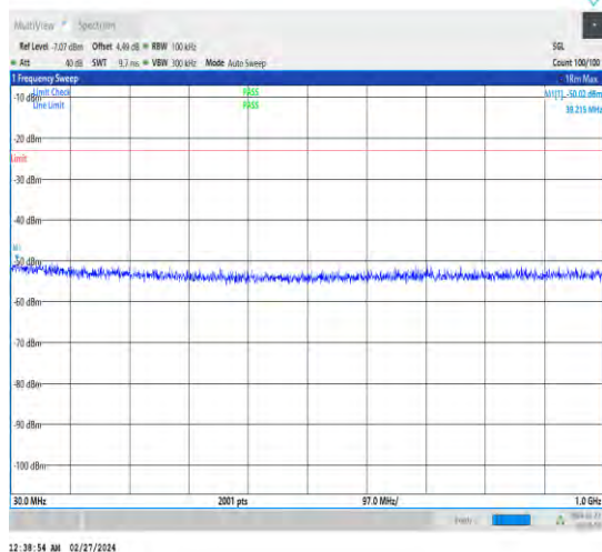
1-N25-15-20-L-1-DFT-PI2BPSK-Inner_1RB_Left-1 @1-30-1000-Ant4-39.22--50.02--23-PASS
