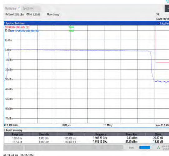
1-N25-15-10-H-6-CP-QPSK-Outer_Full-52@0-Ant4-1-seegraph-PASS-see graph
