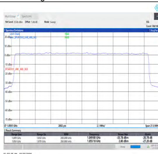
1-N25-15-20-L-3-DFT-PI2BPSK-Outer_Full-100@0-Ant4-1-seegraph-PASS-see graph
