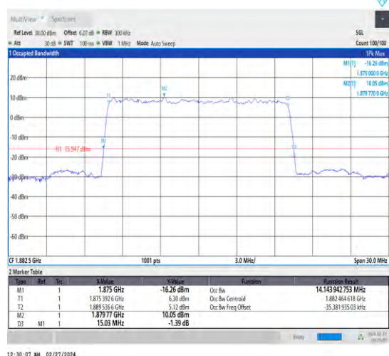
1-N25-15-15-M-9-CP-256QAM-Outer_Full-79@0-Ant 4-14.144-15.030-≤15-PASS
