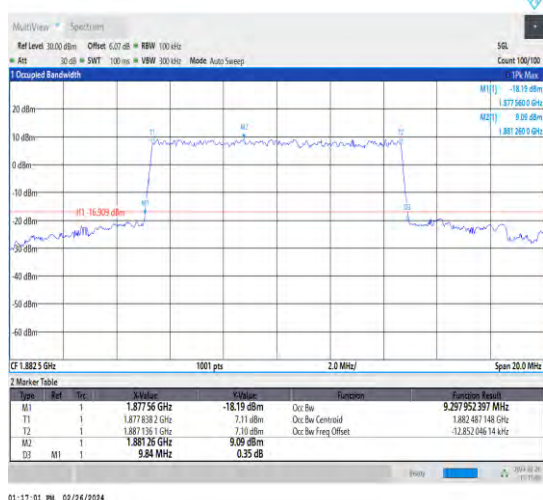
1-N25-15-10-M-7-CP-16QAM-Outer_Full-52@0-Ant 4-9.298-9.840-≤10-PASS
