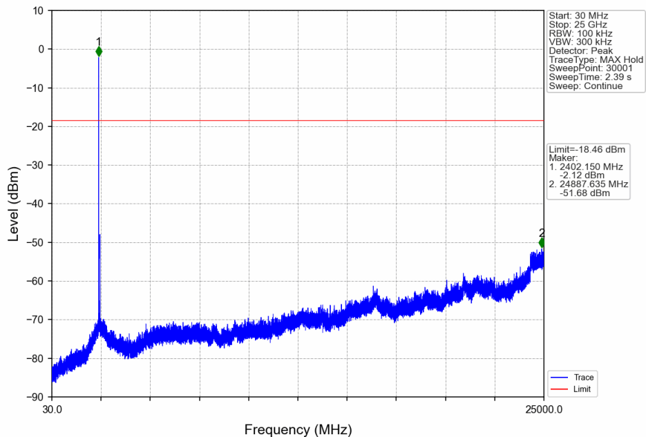
1M_LCH_2402MHz_Ant7_NTNV
