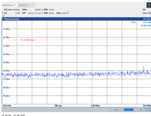
Band26-15MHz-QPSK-26865-1RB#0-Range2:0.15~30MHz
