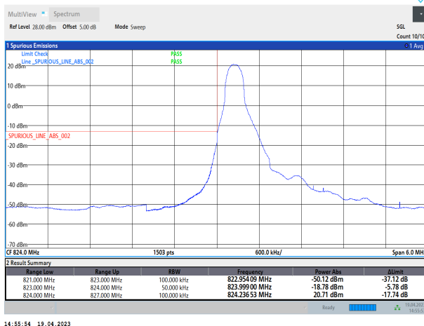
Band26-1.4MHz-QPSK-26797-6RB#0
