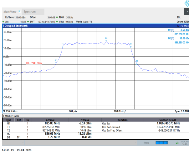
Band26-1.4MHz-QPSK-26915-6RB#0
