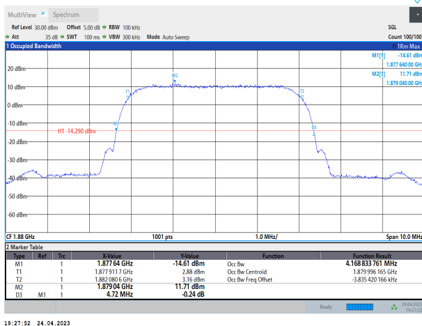
Band2-9400-4.72
