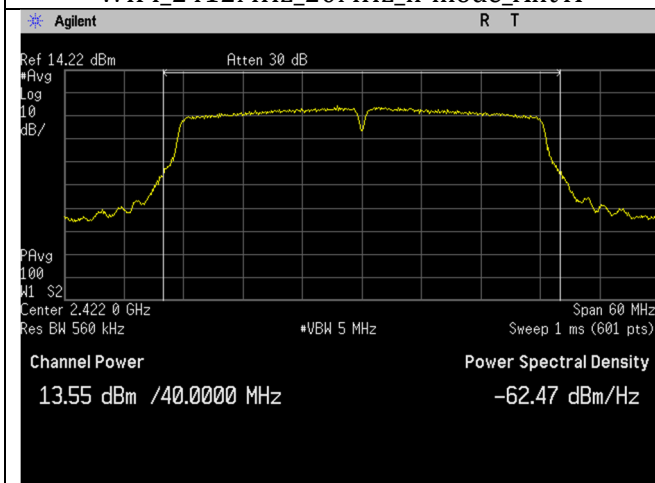
WIFI_2422MHz_40MHz_n-mode_Ant A
