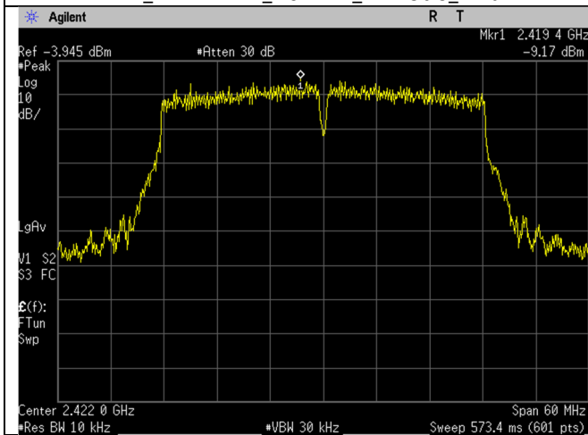
WIFI_2422MHz_40MHz_n-mode_Ant A
