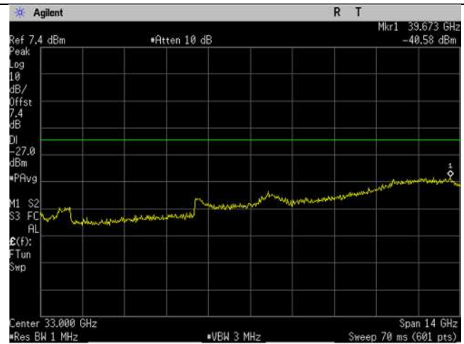
5670MHz_134_40MHz_n-mode_26-40GHz_Ant B
