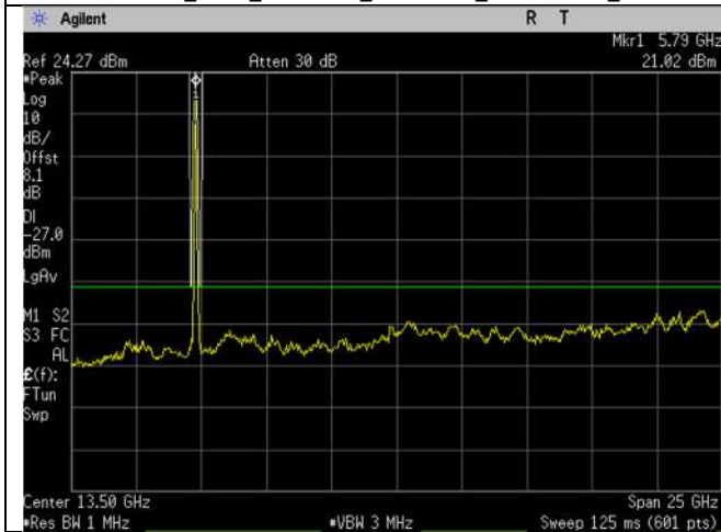
5785MHz_157_20MHz_n-mode_1-26GHz_Ant A
