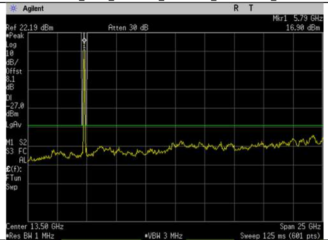
5785MHz_157_20MHz_n-mode_1-26GHz_Ant B
