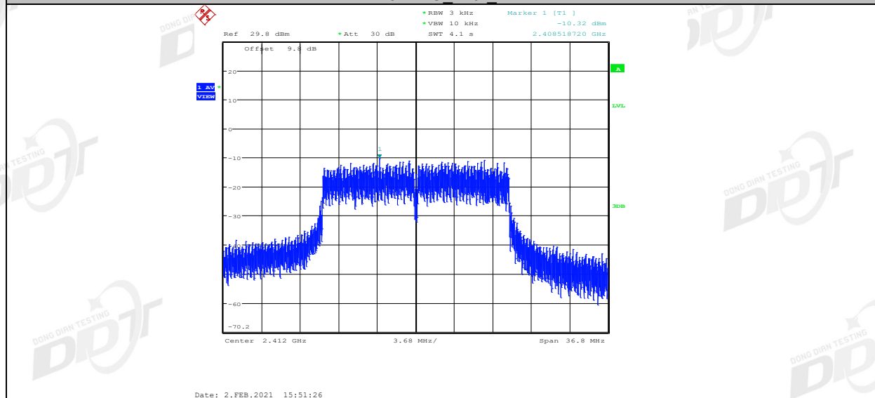
11N20MIMO Ant2 2412
