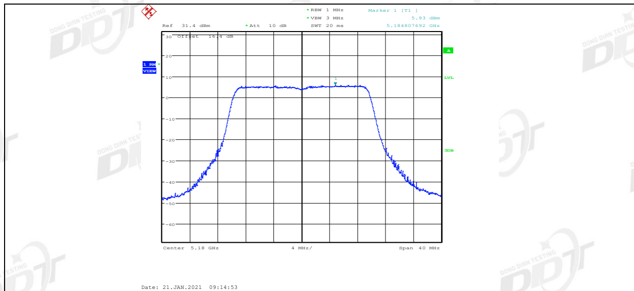
11AX20MIMO Ant2 5180
