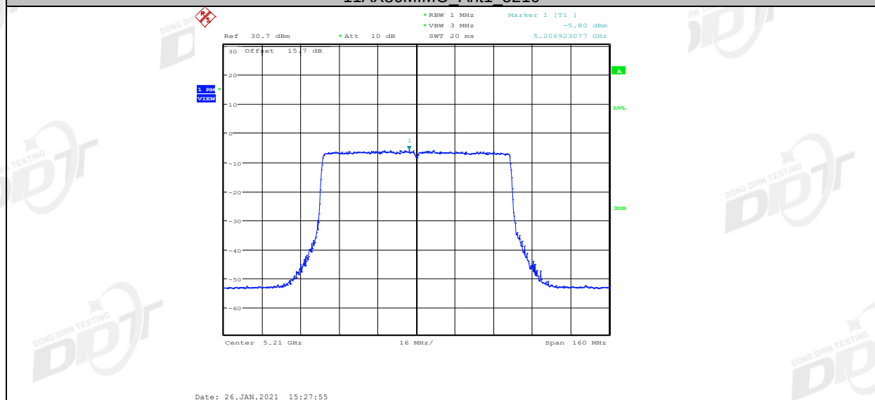
11AX80MIMO Ant2 5210
