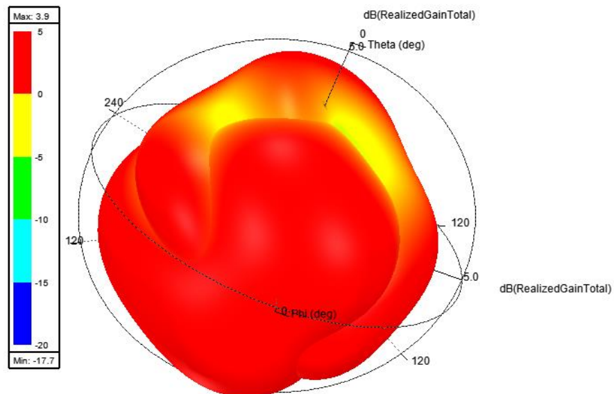
3D patterns @2.4GHz
