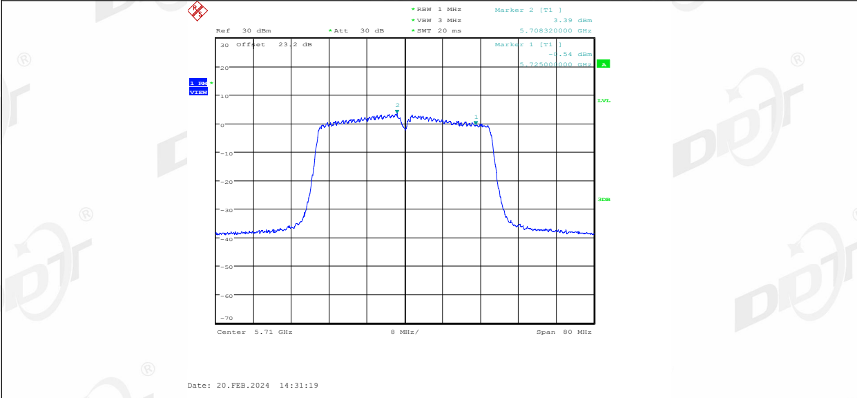
11N40MIMO Ant1_5710_UNII-3
