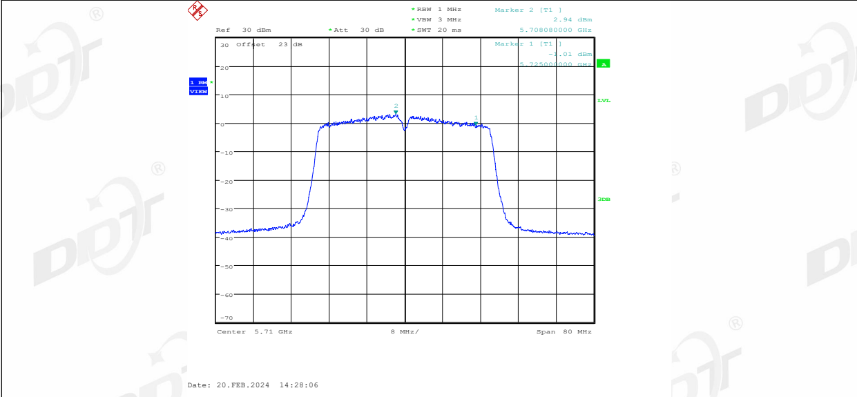
11N40MIMO Ant2_5710_UNII-2C
