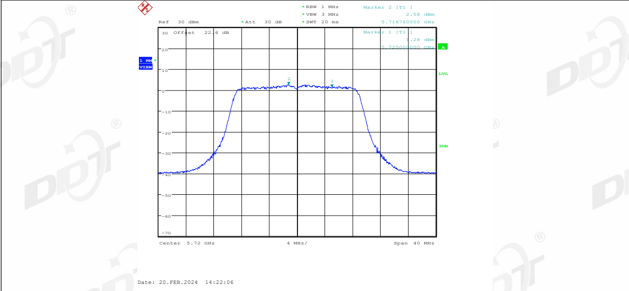
11N20MIMO Ant2_5720_UNII-2C
