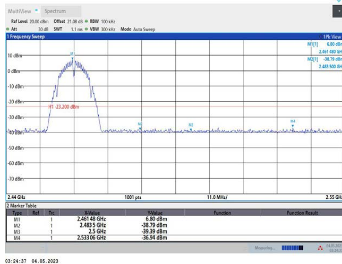
11B_Ant1_High_2462
