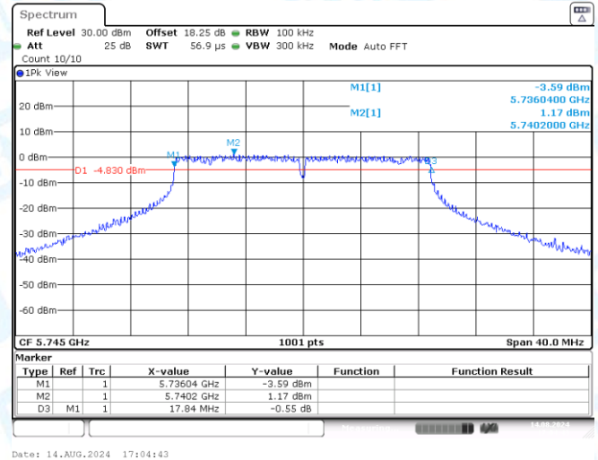
11N20SISO-Ant2-5745-PASS
