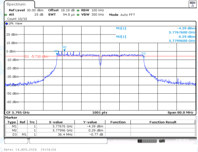
11N40SISO-Ant2-5795-PASS
