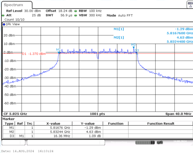
11A-Ant2-5825-PASS
