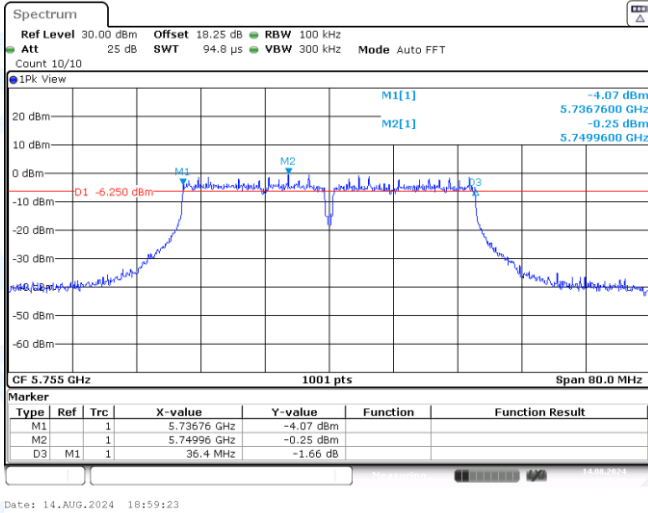
11N40SISO-Ant2-5755-PASS
