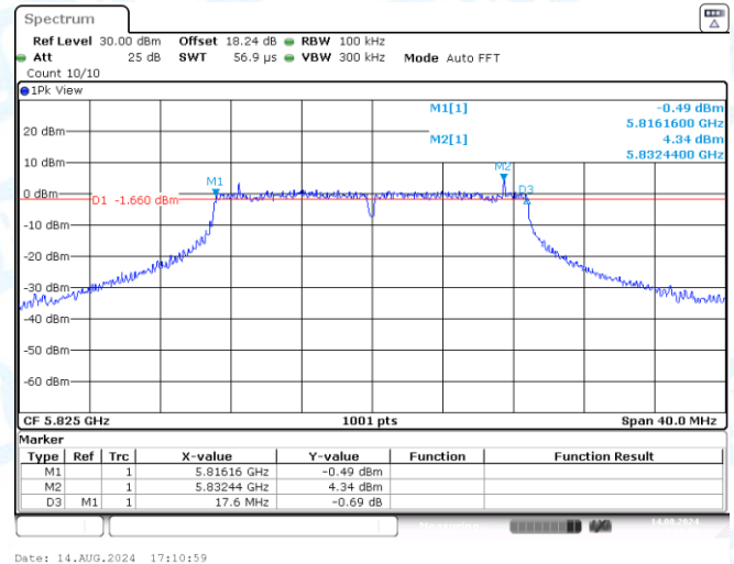
11N20SISO-Ant2-5825-PASS
