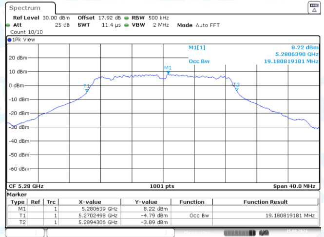
11AC20SISO-Ant2-5280
