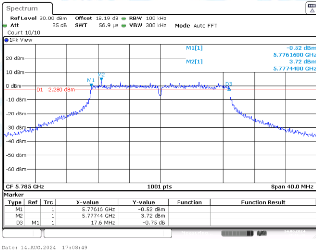
11N20SISO-Ant2-5785-PASS
