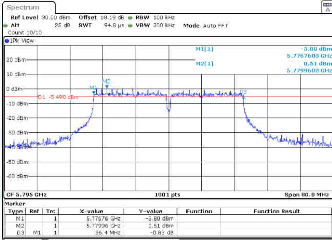
11AC40SISO-Ant2-5795-PASS
