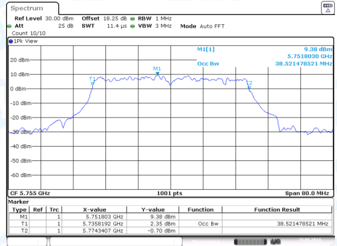
11AX40SISO-Ant2-5755
