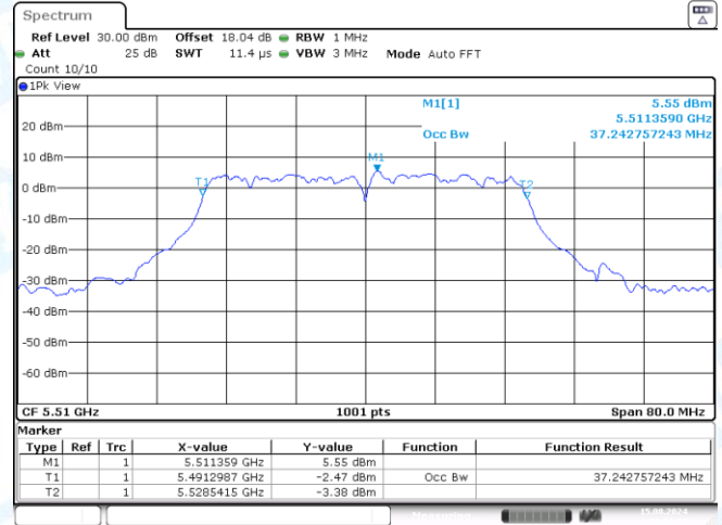
11AC40SISO-Ant2-5510
