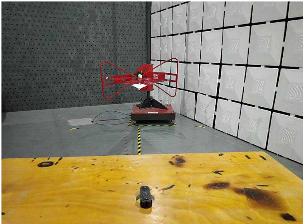
Radiated Emissions, 30MHz to 1GHz Test Setup
