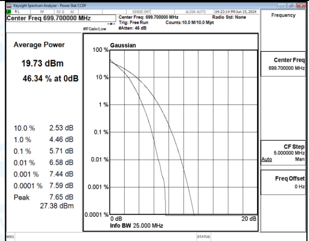
Band12-1.4MHz-QPSK-23095-6RB#0-PASS
