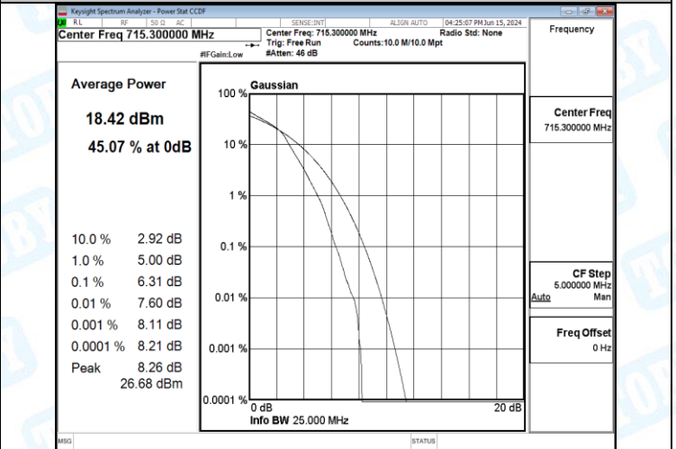
Band12-3MHz-QPSK-23025-15RB#0-PASS
