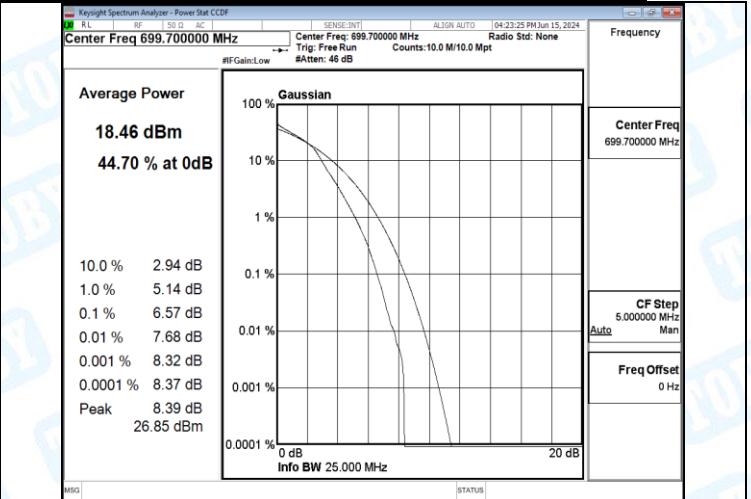
Band12-1.4MHz-16QAM-23095-6RB#0-PASS
