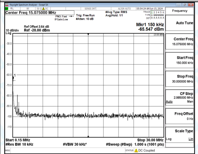
Band12_3MHz_16QAM_23025_1RB#14_1000~3000_1000~3000
