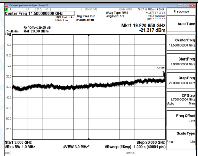
Band2_10MHz_QPSK_19150_50RB#0_0.15~30_0.15~30
