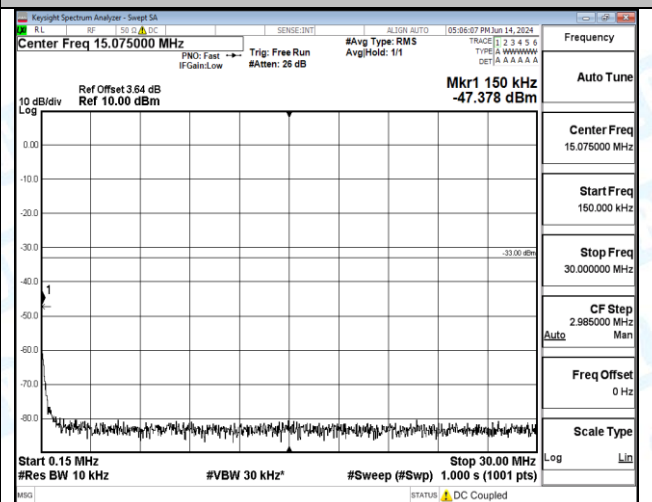
Band2_1.4MHz_16QAM_18900_6RB#0_1000~3000_1000~3000
