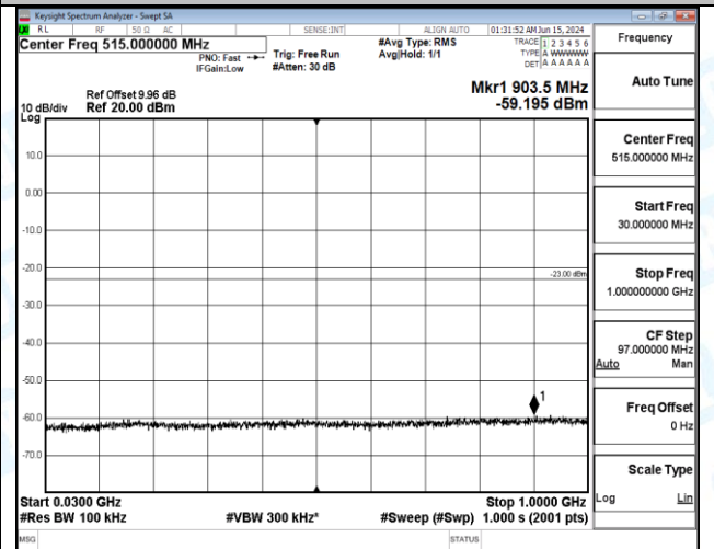
Band4_15MHz_QPSK_20025_1RB#0_3000~20000_3000~20000
