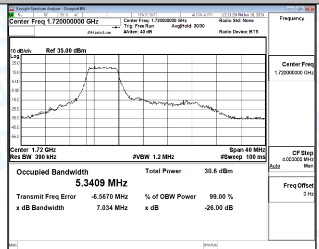
Band4-20MHz-16QAM-20300-27RB#0-PASS
