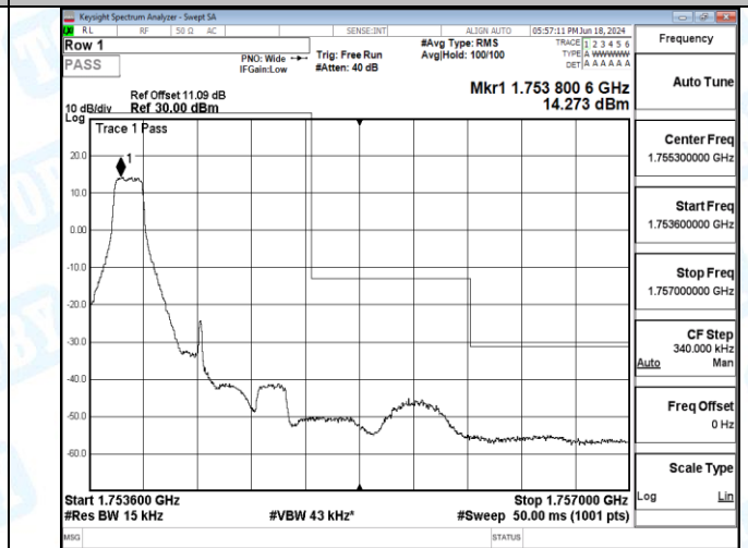
Band4_1.4MHz_16QAM_20393_6RB#0
