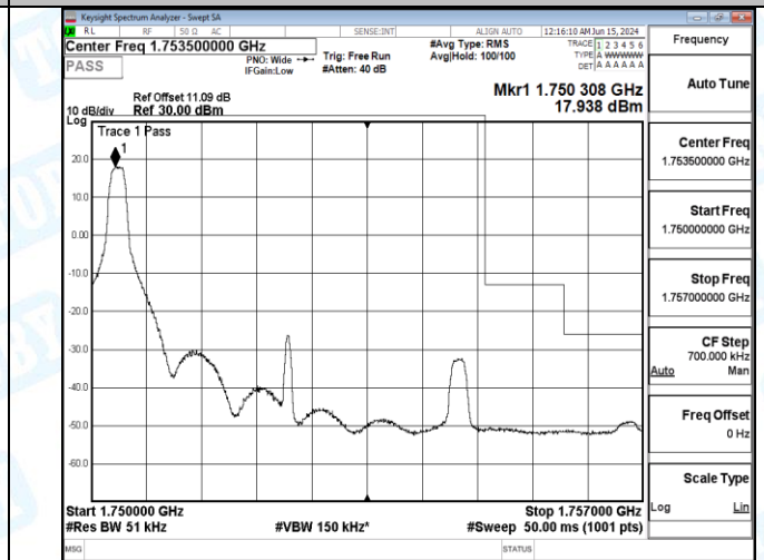
Band4_5MHz_16QAM_20375_25RB#0
