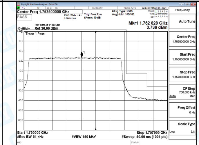
Band4_10MHz_QPSK_20000_1RB#49
