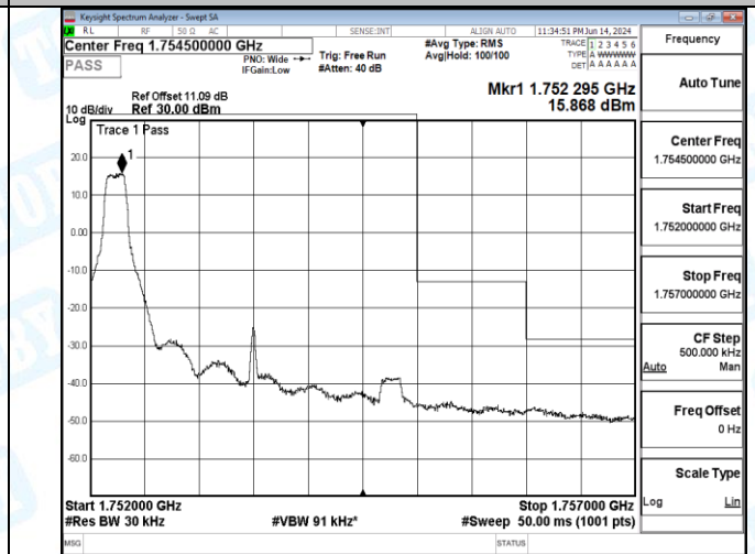
Band4_3MHz_16QAM_20385_15RB#0
