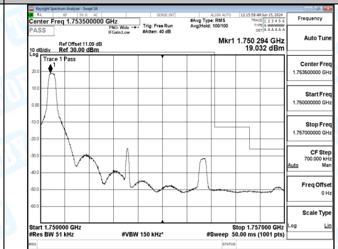
Band4_5MHz_QPSK_20375_25RB#0
