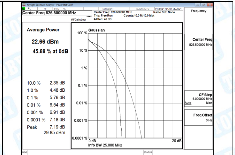
Band5-5MHz-QPSK-20525-25RB#0-PASS
