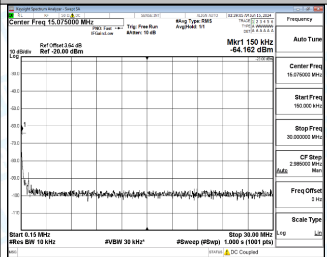
Band5_3MHz_16QAM_20635_1RB#14_1000~3000_1000~3000
