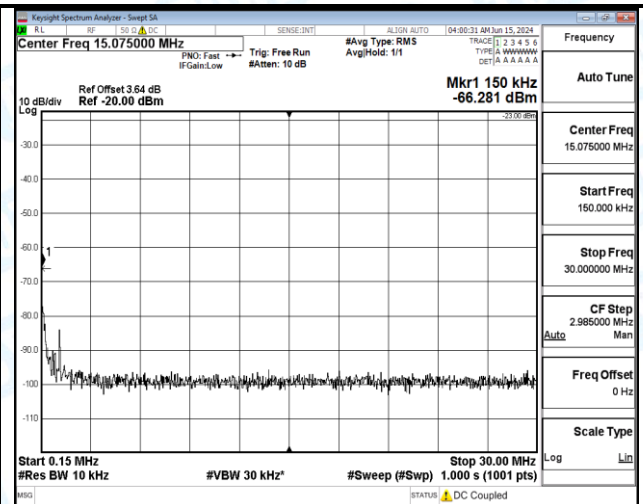
Band5_5MHz_QPSK_20425_1RB#0_1000~3000_1000~3000
