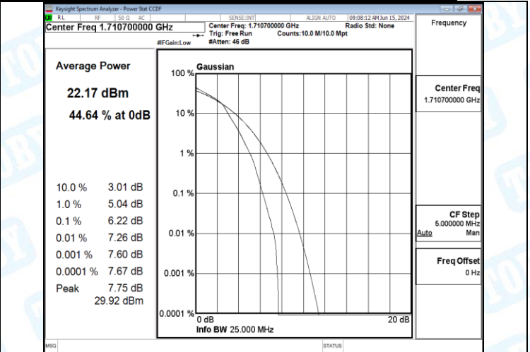
Band66-1.4MHz-16QAM-132322-6RB#0-PASS
