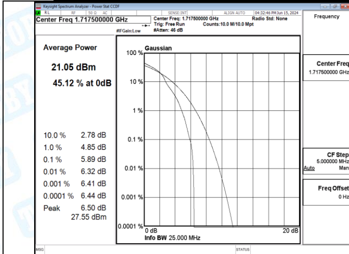
Band66-15MHz-16QAM-132322-1RB#0-PASS
