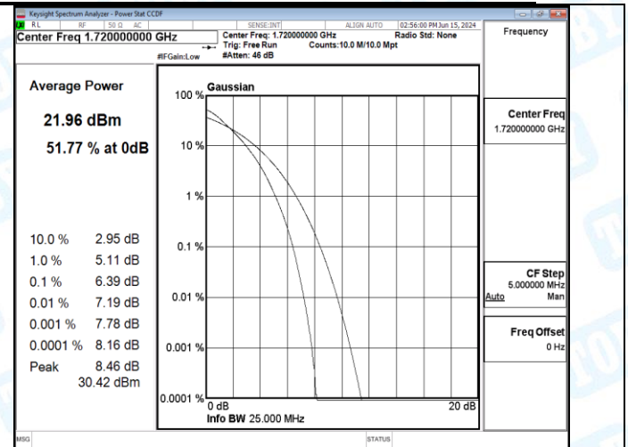
Band66-20MHz-QPSK-132322-100RB#0-PASS
