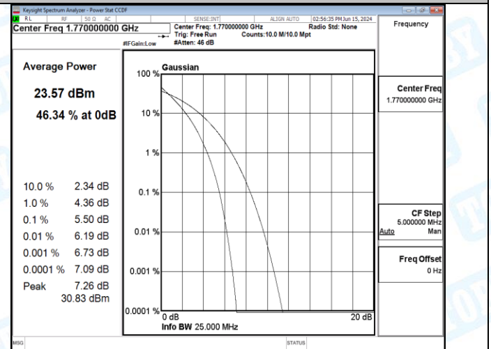
Band66-20MHz-16QAM-132072-27RB#0-PASS
