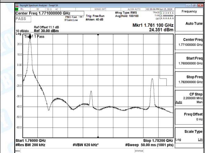
Band66_20MHz_QPSK_132572_100RB#0
