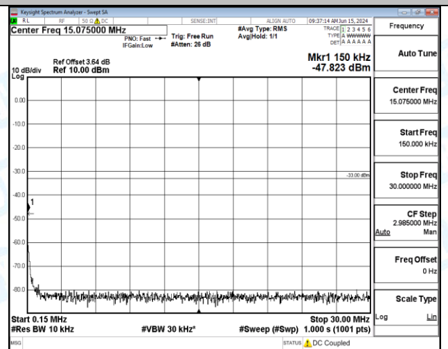
Band66_3MHz_QPSK_132657_15RB#0_1000~3000_1000~3000
