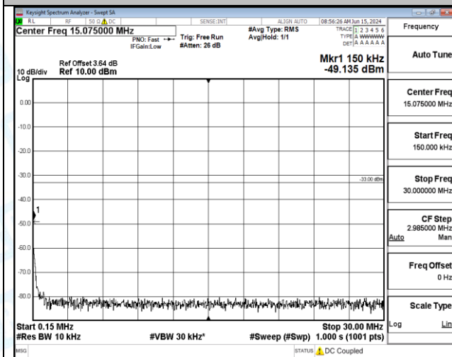
Band66_1.4MHz_16QAM_132665_1RB#0_1000~3000_1000~3000
