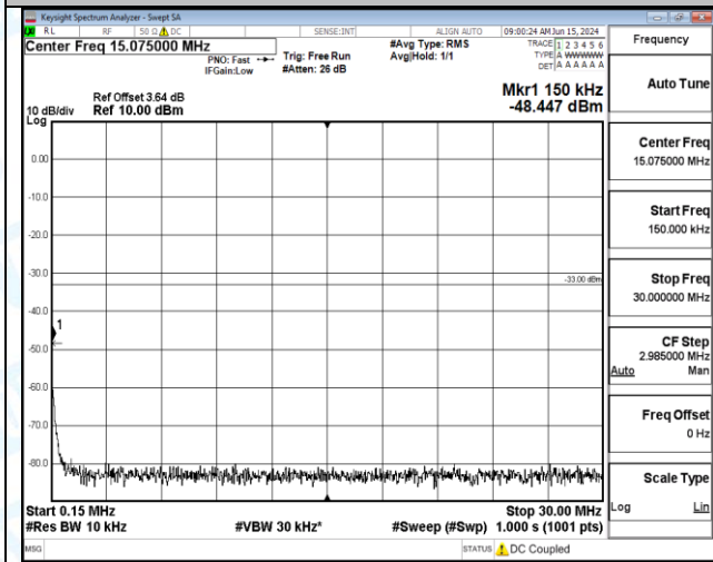
Band66_1.4MHz_16QAM_132665_6RB#0_1000~3000.1000~3000
