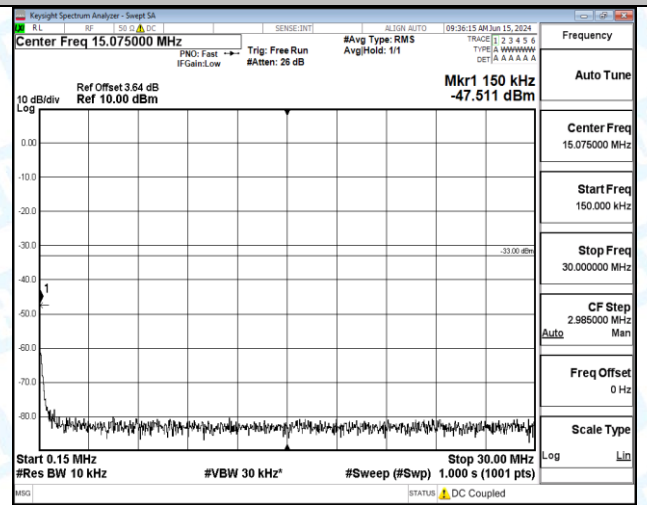
Band66_3MHz_16QAM_132657_1RB#14_1000-3000_1000-3000
