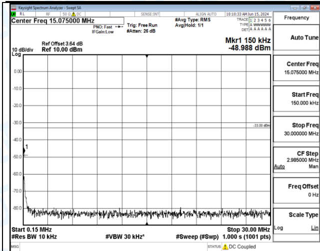
Band66_5MHz_QPSK_131997_1RB#24_1000~3000_1000~3000
