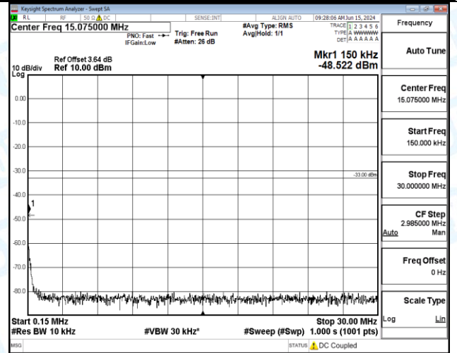
Band66_3MHz_16QAM_132322_1RB#0_1000~3000_1000~3000
