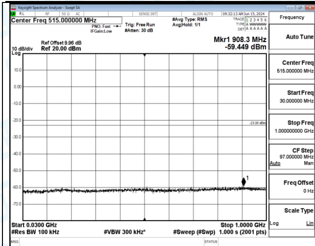
Band66_3MHz_16QAM_132322_15RB#0_3000~20000_3000~20000
