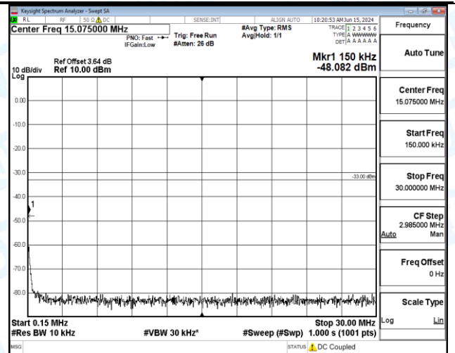
Band66_5MHz_QPSK_132647_1RB#0_1000-3000_1000-3000
