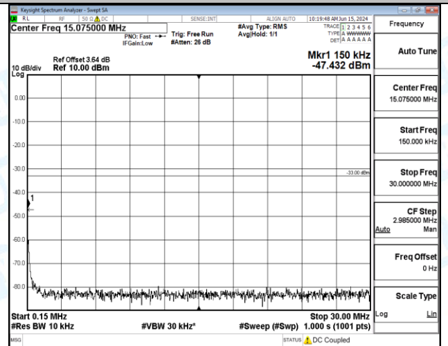
Band66_5MHz_16QAM_132322_25RB#0_1000~3000_1000~3000
