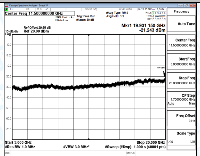
Band66_5MHz_QPSK_132647_25RB#0_0.15~30_0.15~30
