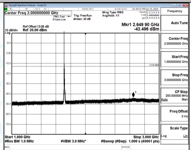
Band66_10MHz_QPSK_132022_1RB#49_0.009~0.15_0.009~0.15
