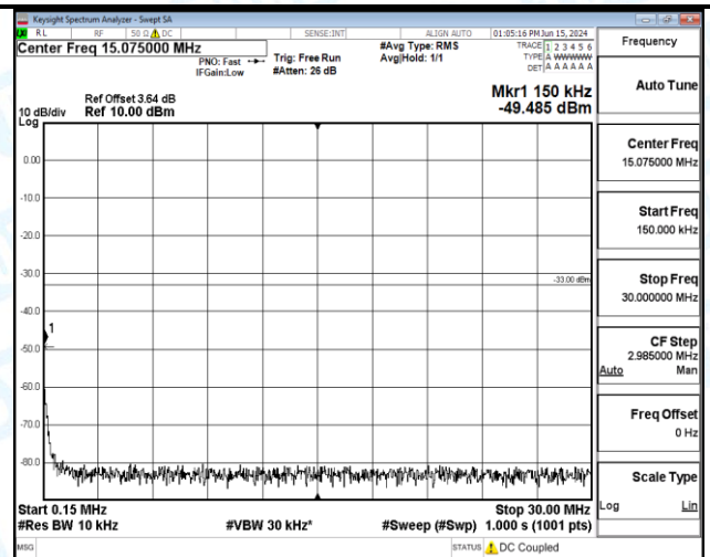
Band66_10MHz_QPSK_132022_1RB#0_1000~3000_1000~3000
