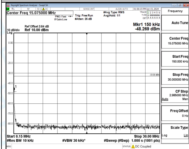
Band66_10MHz_16QAM_132022_1RB#0_1000~3000_1000~3000
