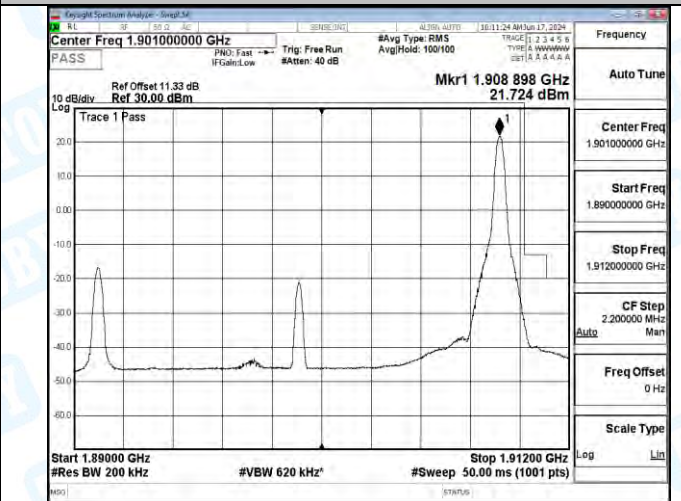
Band2_20MHz_16QAM_19100_1RB#99
