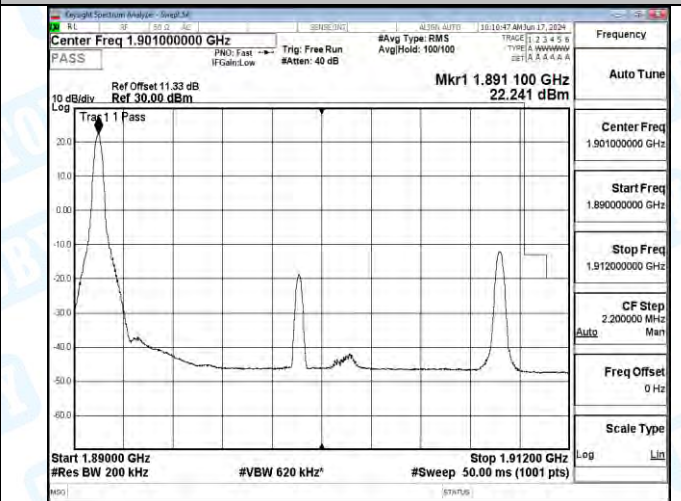
Band2_20MHz_QPSK_19100_100RB#0
