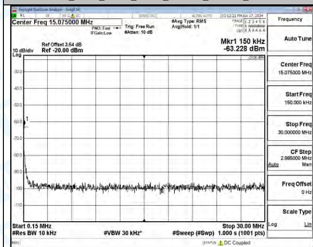
Band5_5MHz_QPSK_20525_25RB#0_1000~3000_1000~3000
