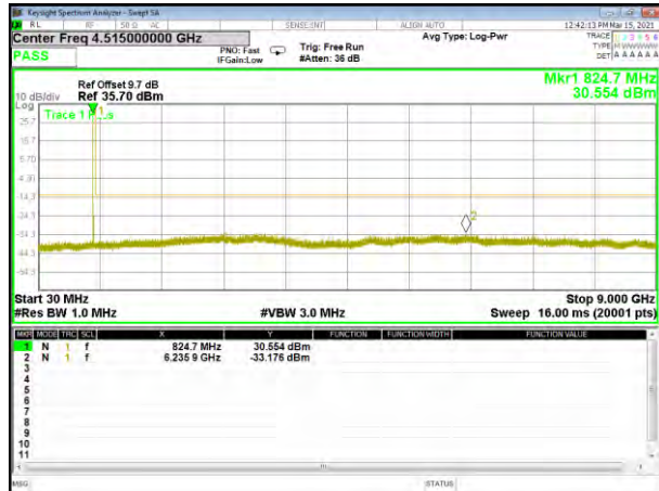
GPRS850 Low
