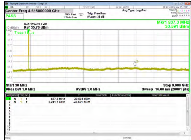
GPRS850 Middle
