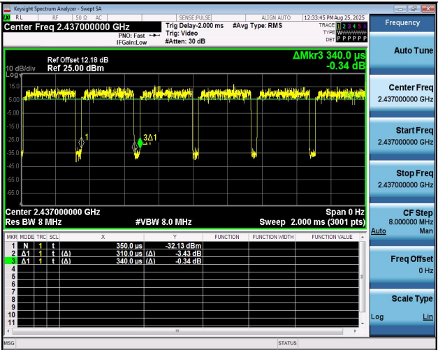
NTNV-11BE40MIMO-Ant2-2437
