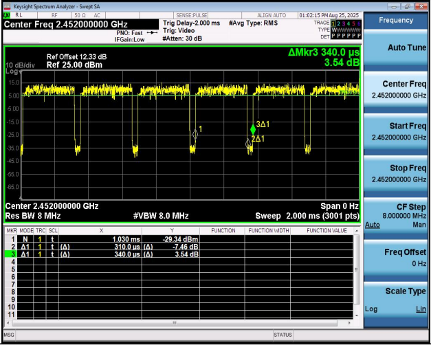
NTNV-11BE40MIMO-Ant2-2452
