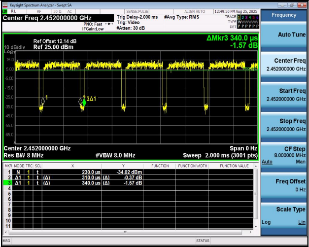
NTNV-11BE40MIMO-Ant1-2452
