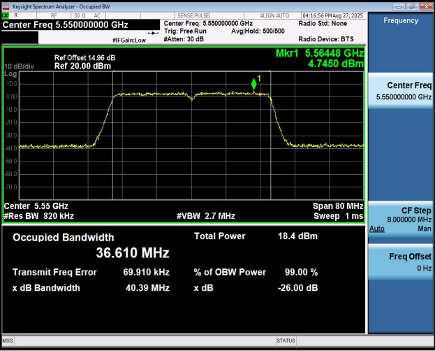
11AC40MIMO-Ant2-5550
