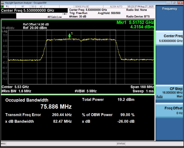
11AC80MIMO-Ant2-5530
