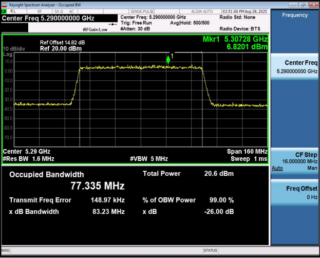
11AX80MIMO-Ant2-5290
